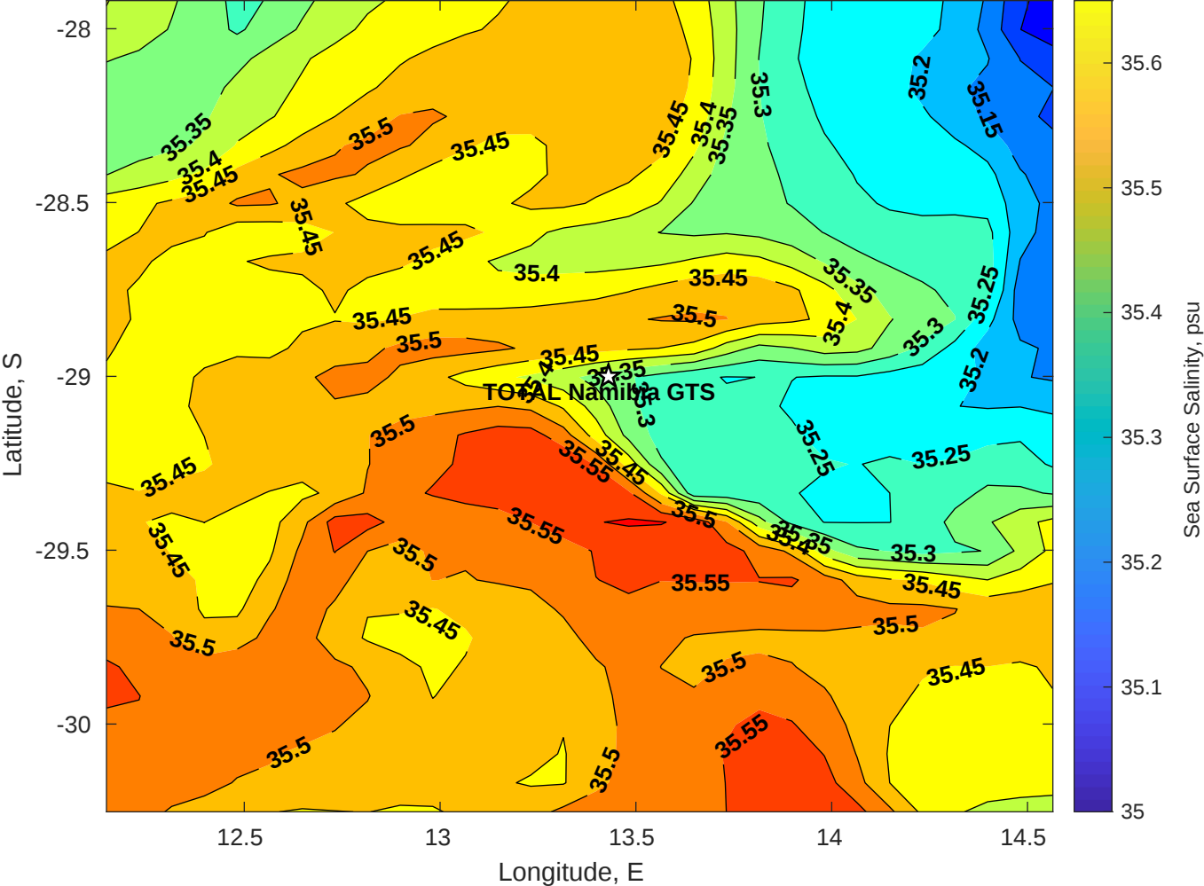
Surface Salinity for TOTAL Namibia GTS at 14-Apr-2025 00:00:00
