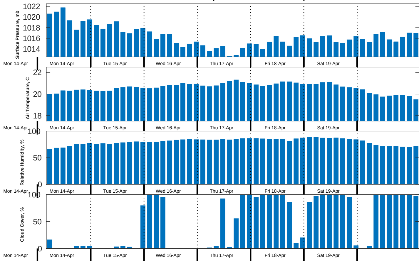
Met Forecast for TOTAL Namibia GTS from 15-Apr-2025 00:00:00 to 22-Apr-2025 00:00:00
