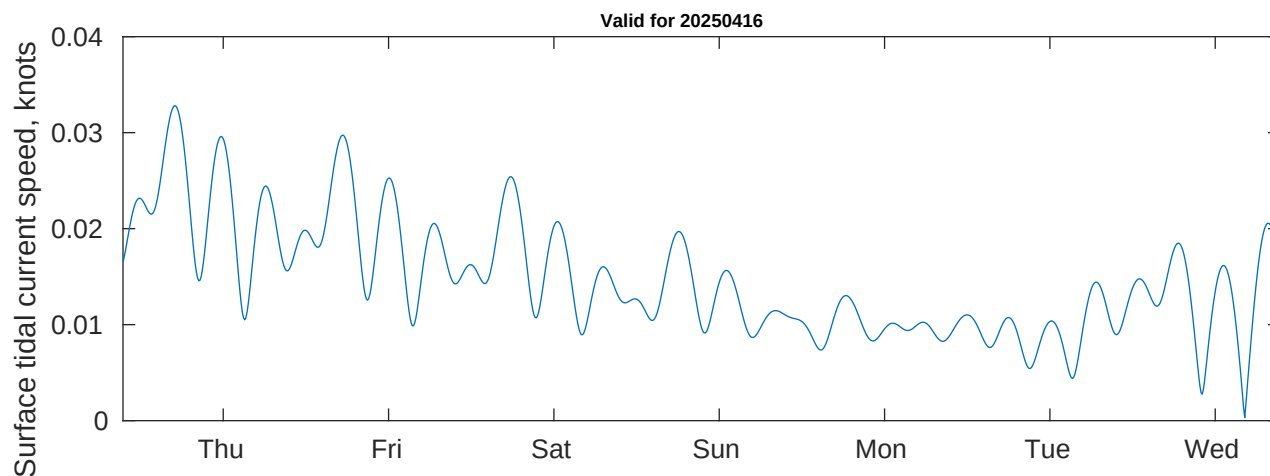
Tidal Currents and Heights for Benthic Solutions South Africa HF Site1 at 20250416
