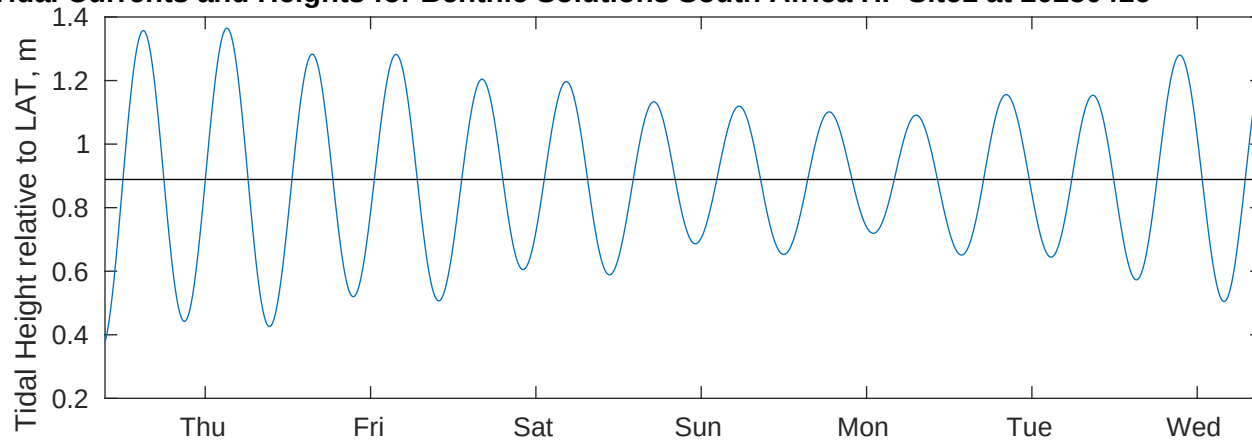
Tidal Currents and Heights for Benthic Solutions South Africa HF Site1 at 20250416
