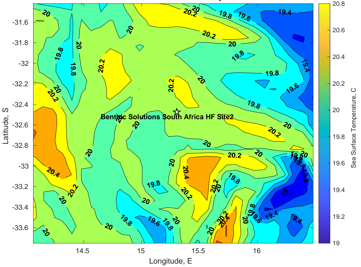
SST for Benthic Solutions South Africa HF Site2 at 15-Apr-2025 00:00:00
