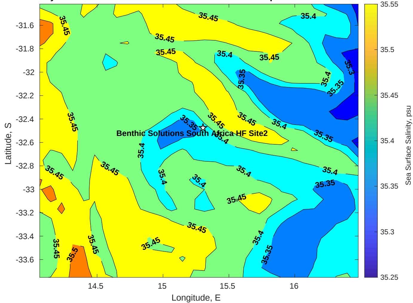
Surface Salinity for Benthic Solutions South Africa HF Site2 at 15-Apr-2025 00:00:00
