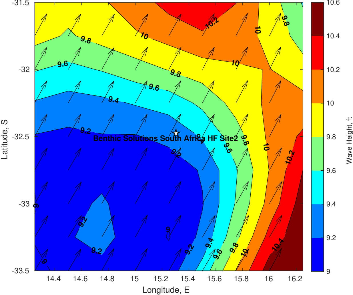
Wave Height (ft) for Benthic Solutions South Africa HF Site2 at 16-Apr-2025 09:00:00
