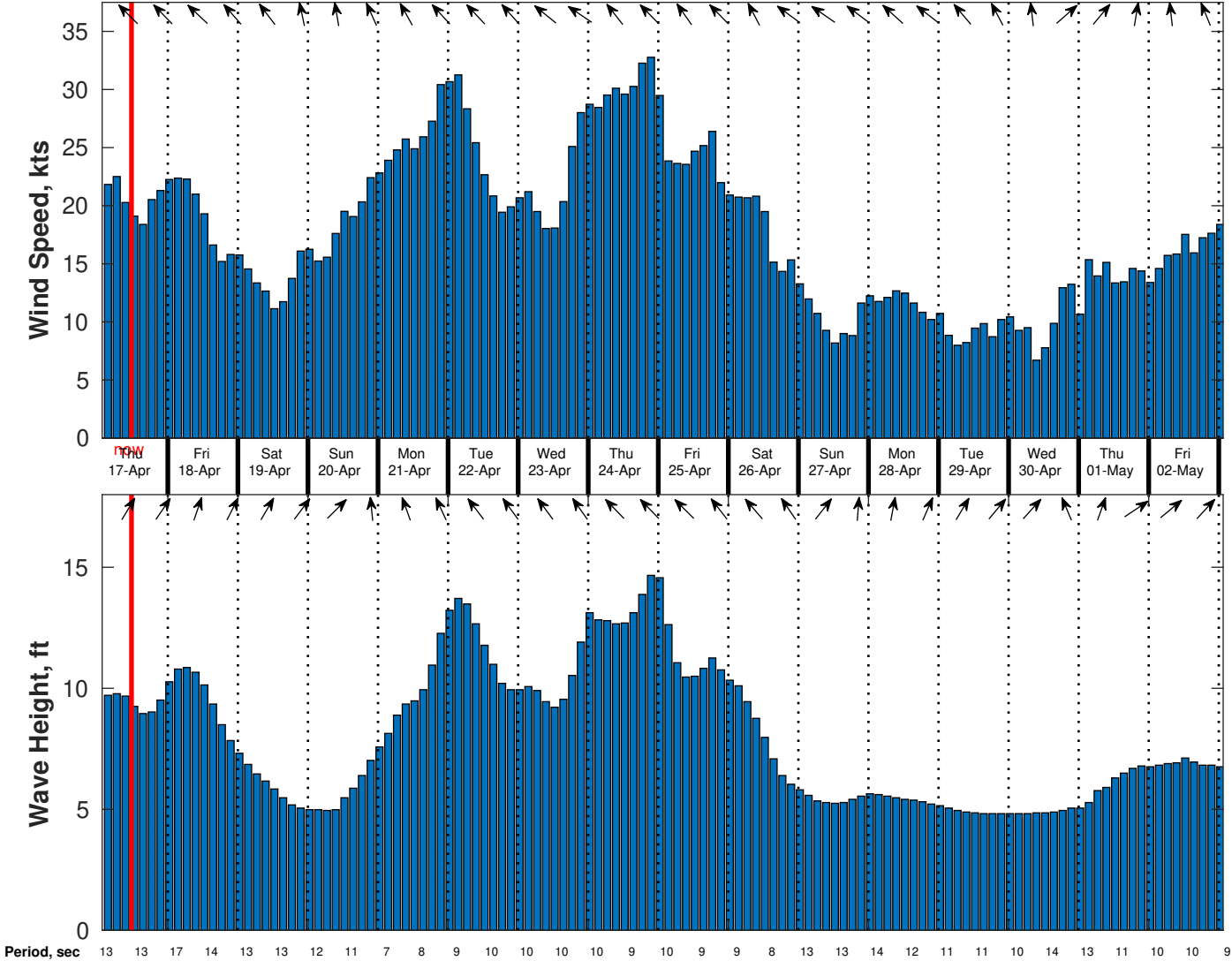
Wind & Wave Forecast for Benthic Solutions South Africa HF Site2 from 16-Apr-2025 02:00:00 to 02-May-2025 02:00:00
