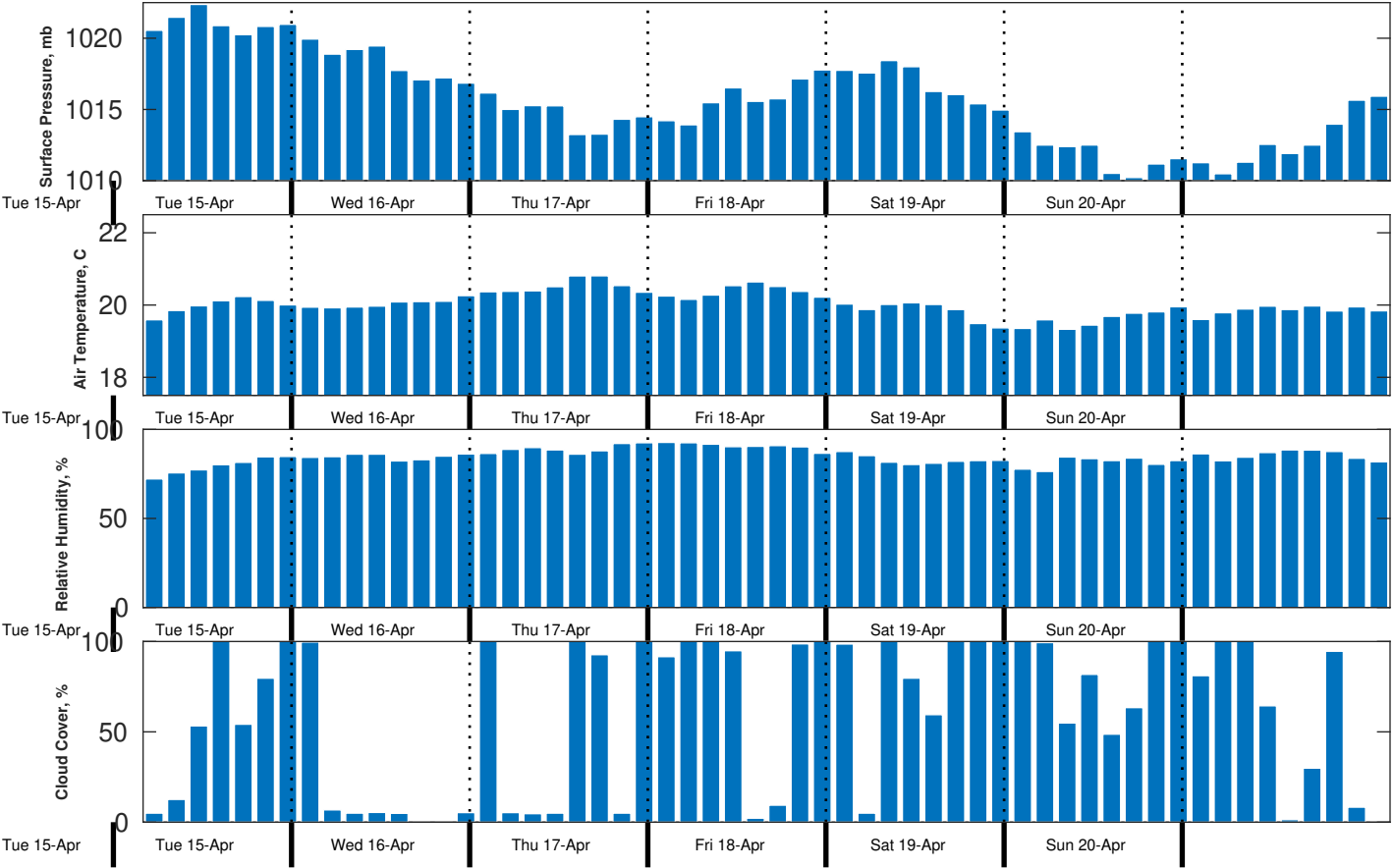
Met Forecast for Benthic Solutions South Africa HF Site2 from 16-Apr-2025 00:00:00 to 23-Apr-2025 00:00:00
