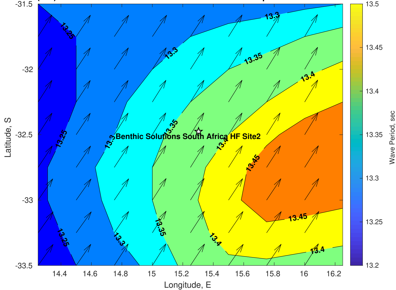
Wave Period (sec) for Benthic Solutions South Africa HF Site2 at 16-Apr-2025 09:00:00
