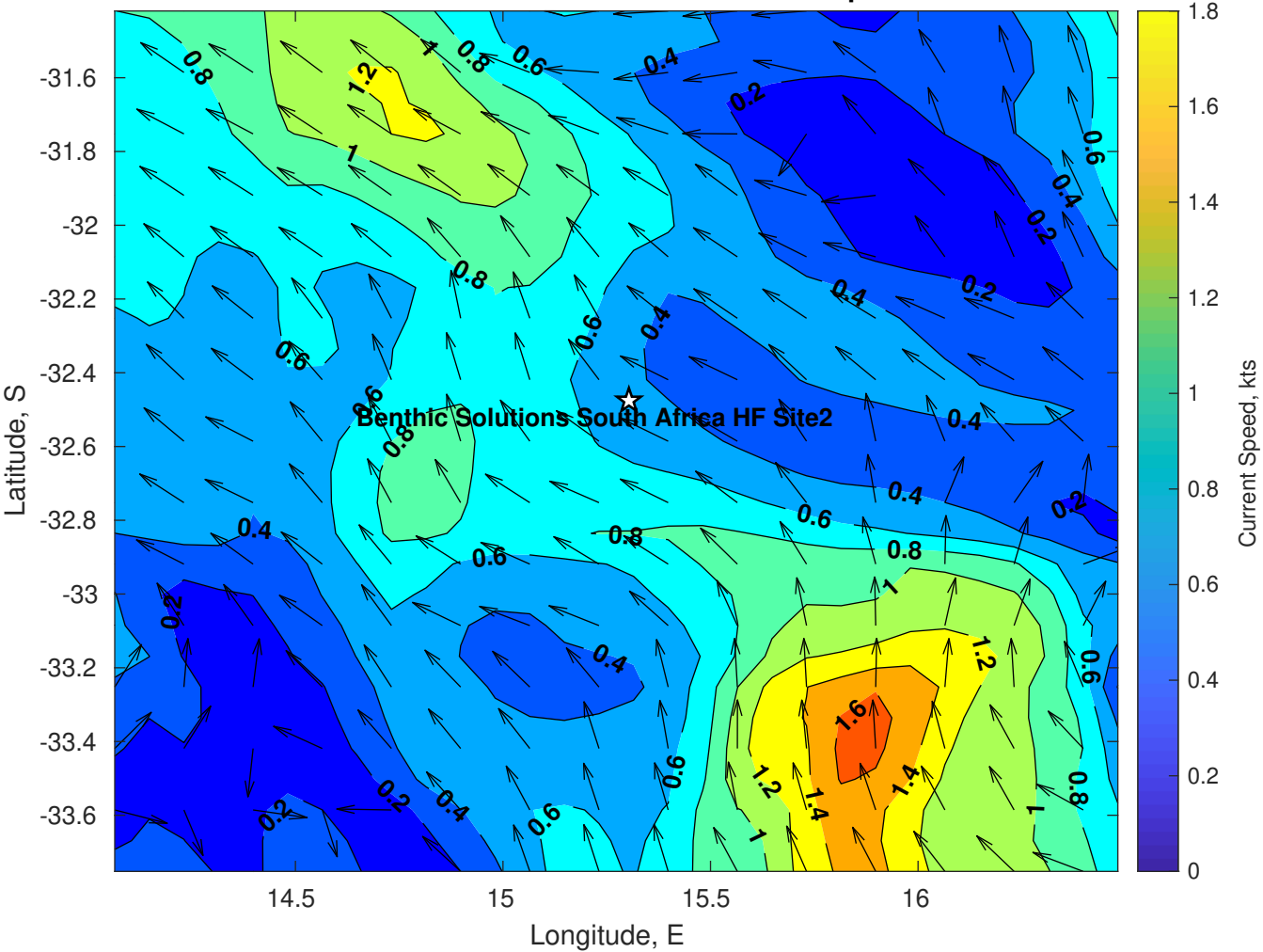
Surface Currents for Benthic Solutions South Africa HF Site2 at 15-Apr-2025 00:00:00
