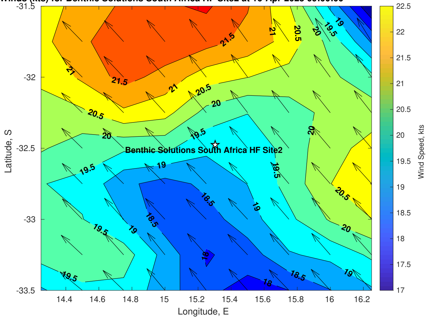
Winds (kts) for Benthic Solutions South Africa HF Site2 at 16-Apr-2025 09:00:00
