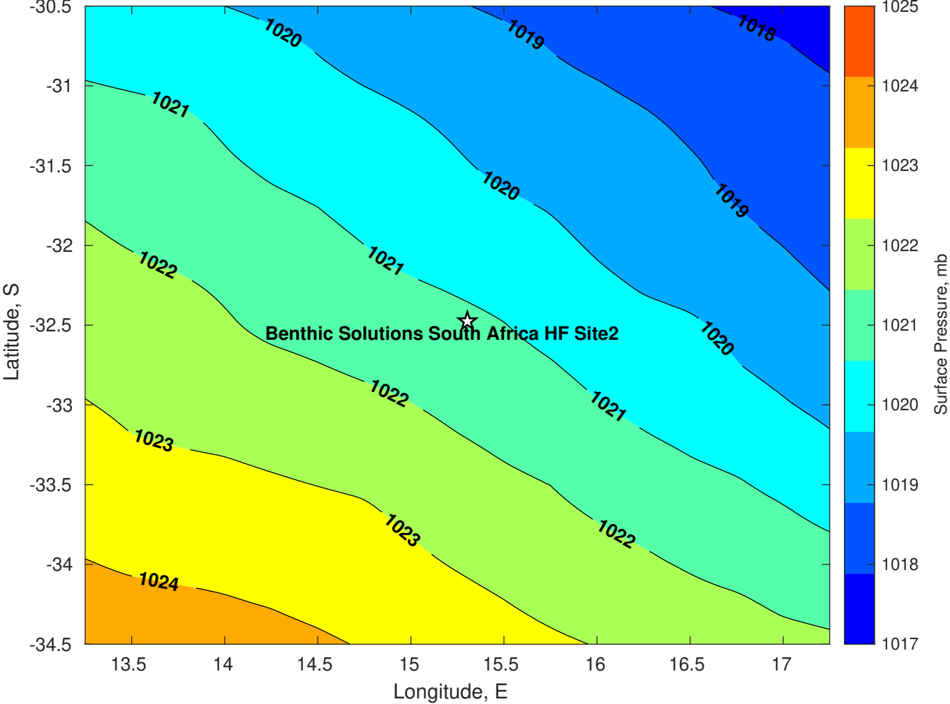
Surface Pressure (mb) for Benthic Solutions South Africa HF Site2 at 16-Apr-2025 00:00:00
