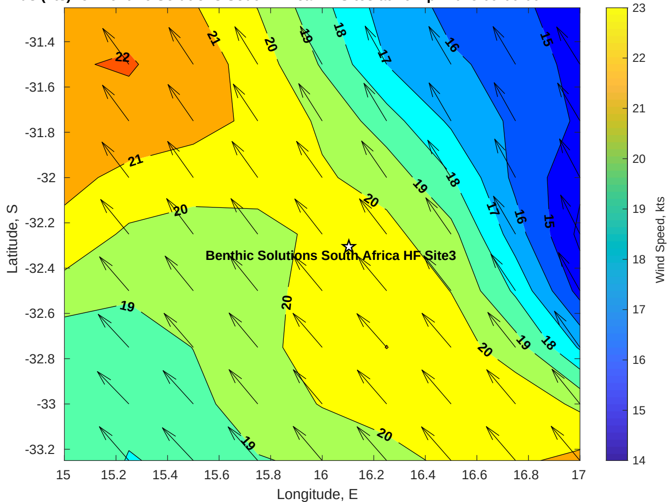
Winds (kts) for Benthic Solutions South Africa HF Site3 at 16-Apr-2025 09:00:00
