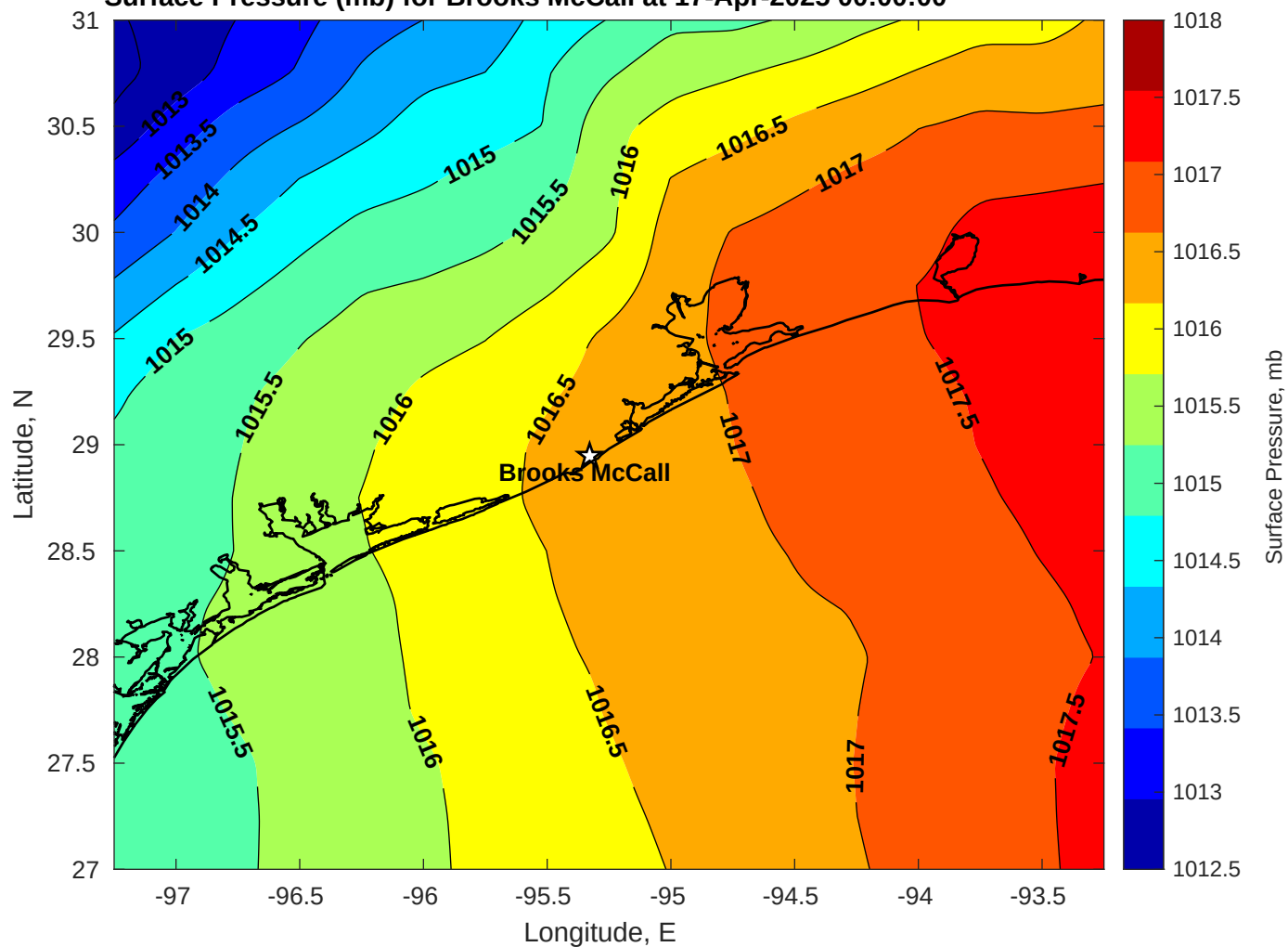
Surface Pressure (mb) for Brooks McCall at 17-Apr-2025 00:00:00
