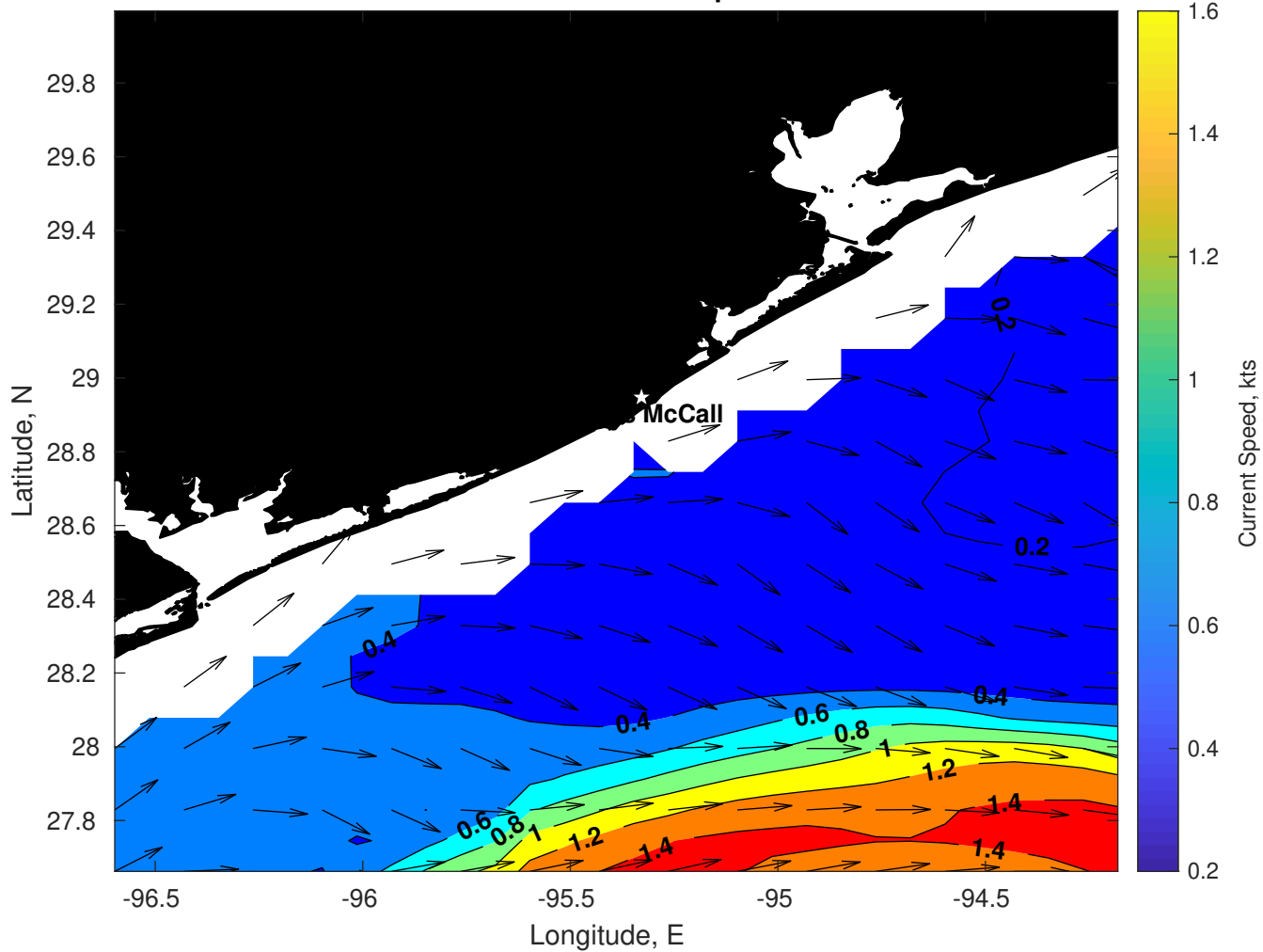
Surface Currents for Brooks McCall at 15-Apr-2025 00:00:00
