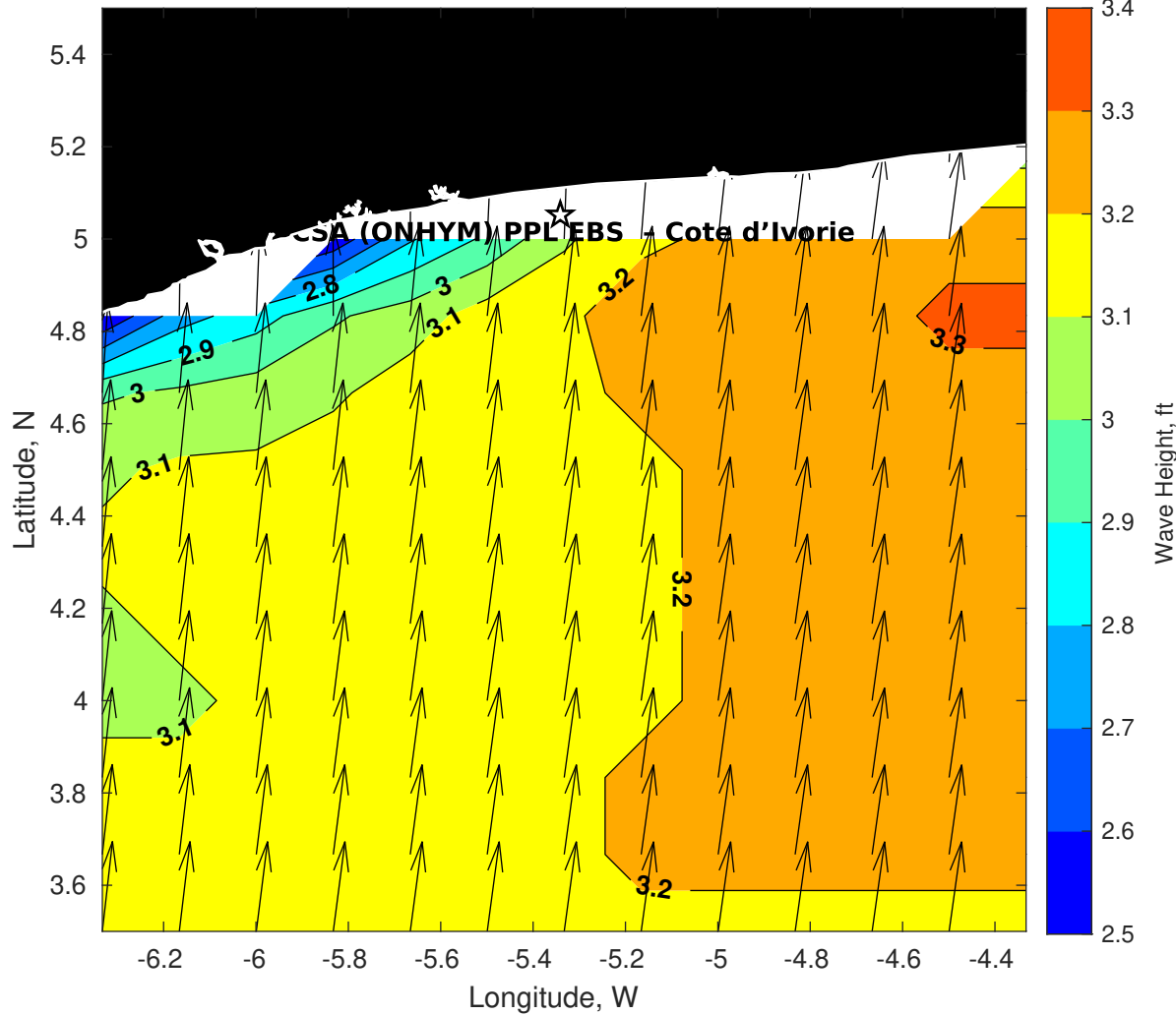
Wave Height (ft) for CSA (ONHYM) PPL EBS - Cote d'Ivoire at 16-Apr-2025 09:00:00
