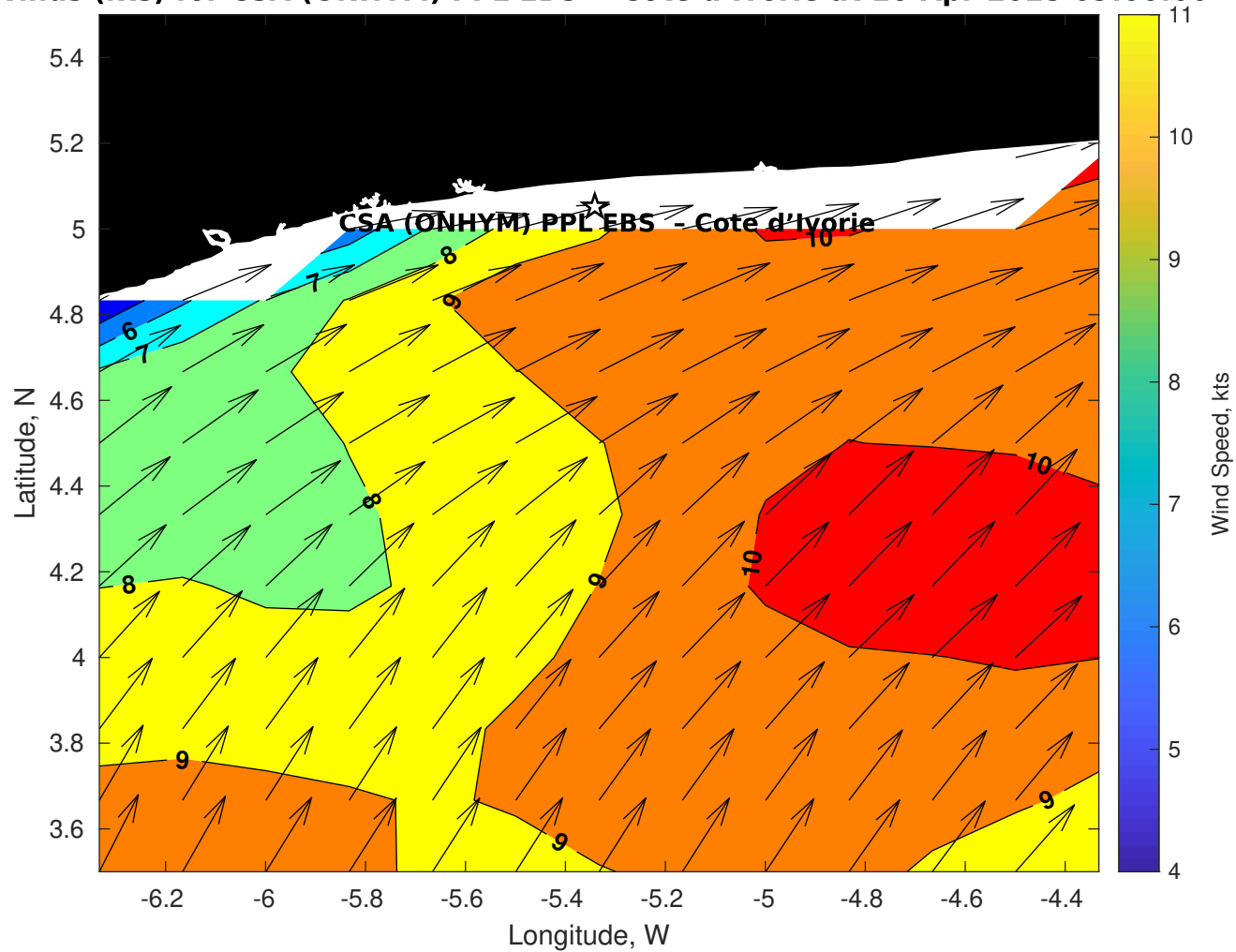
Winds (kts) for CSA (ONHYM) PPL EBS - Cote d'Ivoire at 16-Apr-2025 09:00:00
