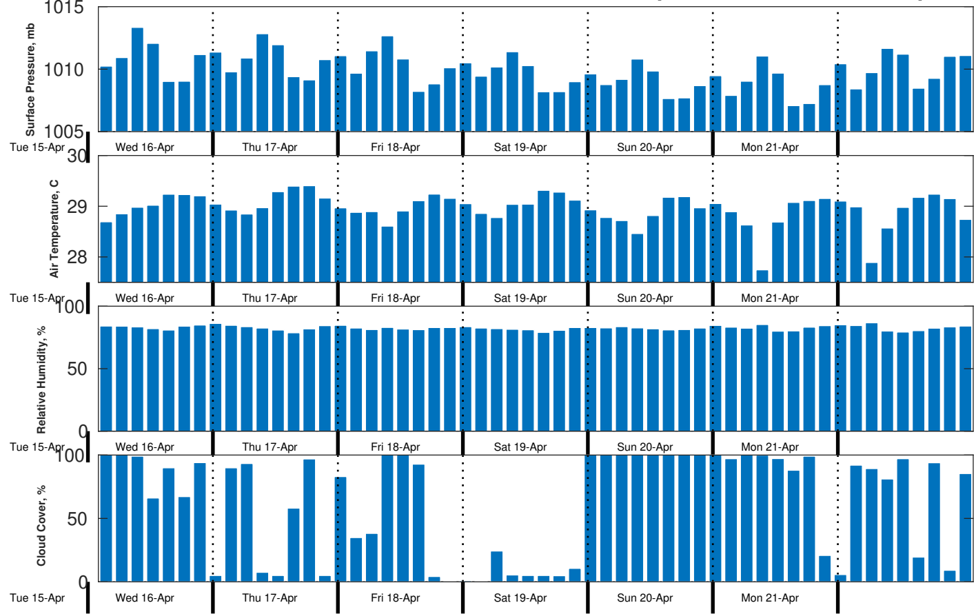
Met Forecast for CSA (ONHYM) PPL EBS - Cote d'Ivoire from 16-Apr-2025 00:00:00 to 23-Apr-2025 00:00:00
