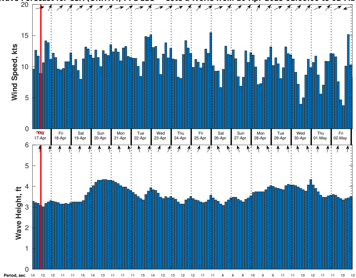
Wind & Wave Forecast for CSA (ONHYM) PPL EBS - Cote d'Ivoire from 16-Apr-2025 01:00:00 to 02-May-2025 01:00:00
