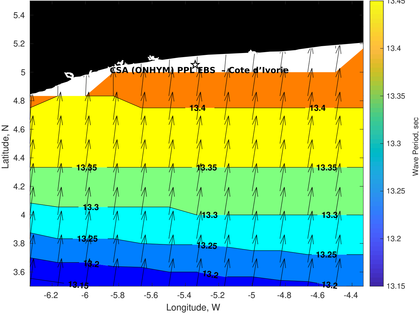
Wave Period (sec) for CSA (ONHYM) PPL EBS - Cote d'Ivoire at 16-Apr-2025 09:00:00
