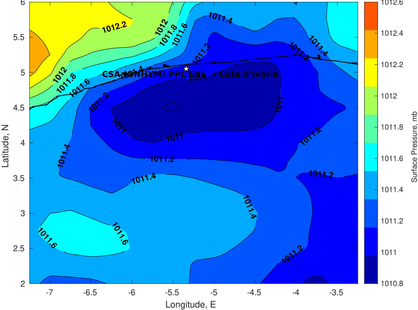
Surface Pressure (mb) for CSA (ONHYM) PPL EBS - Cote d'Ivoire at 18-Apr-2025 00:00:00
