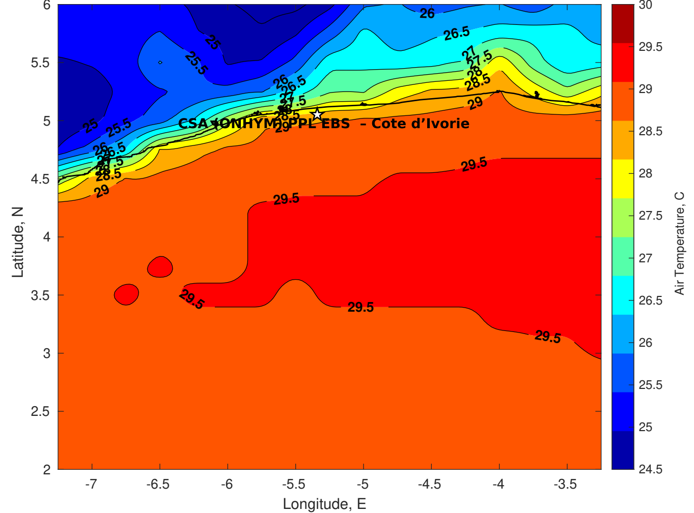
Air Temperature (C) for CSA (ONHYM) PPL EBS - Cote d'Ivoire at 16-Apr-2025
