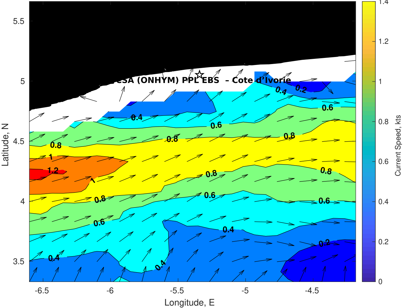
Surface Currents for CSA (ONHYM) PPL EBS - Cote d'Ivoire at 15-Apr-2025 00:00:00
