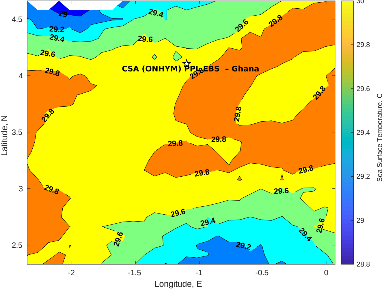
SST for CSA (ONHYM) PPL EBS - Ghana at 15-Apr-2025 00:00:00
