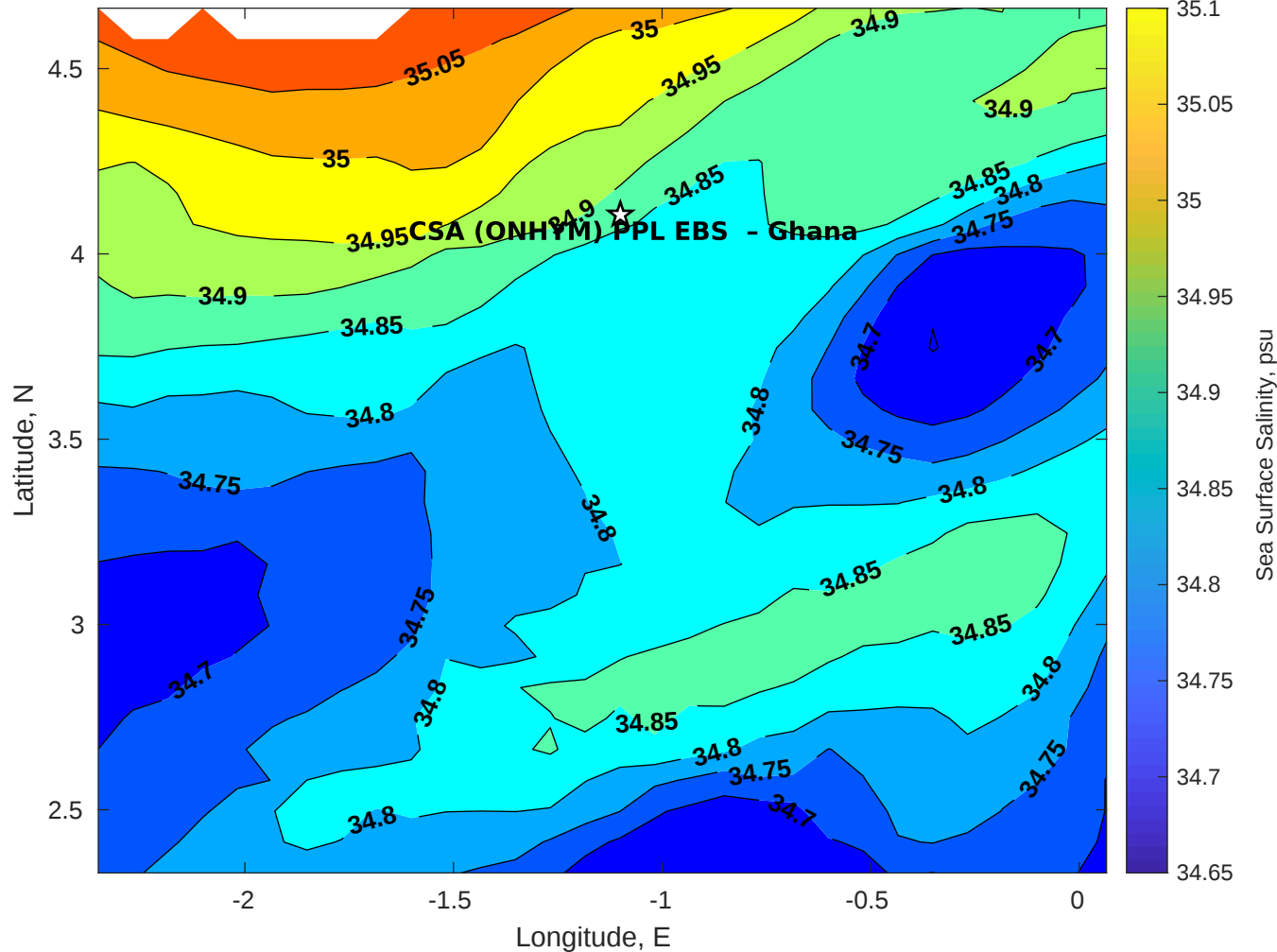
Surface Salinity for CSA (ONHYM) PPL EBS - Ghana at 15-Apr-2025 00:00:00
