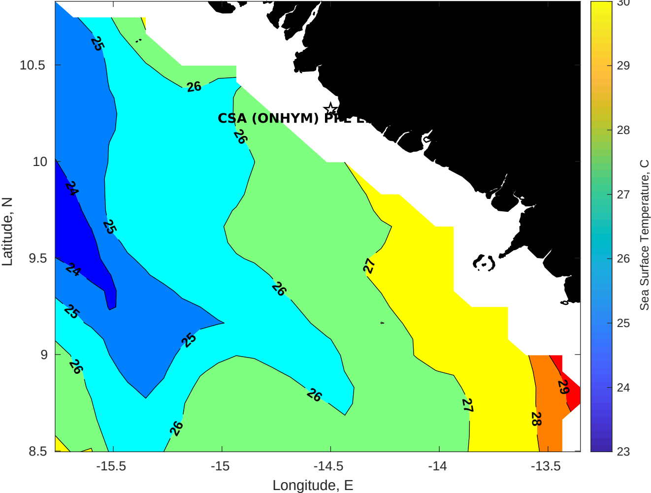
SST for CSA (ONHYM) PPL EBS - Guinea at 15-Apr-2025 00:00:00
