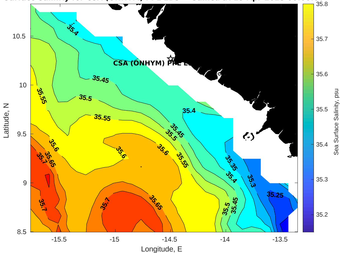
Surface Salinity for CSA (ONHYM) PPL EBS - Guinea at 15-Apr-2025 00:00:00
