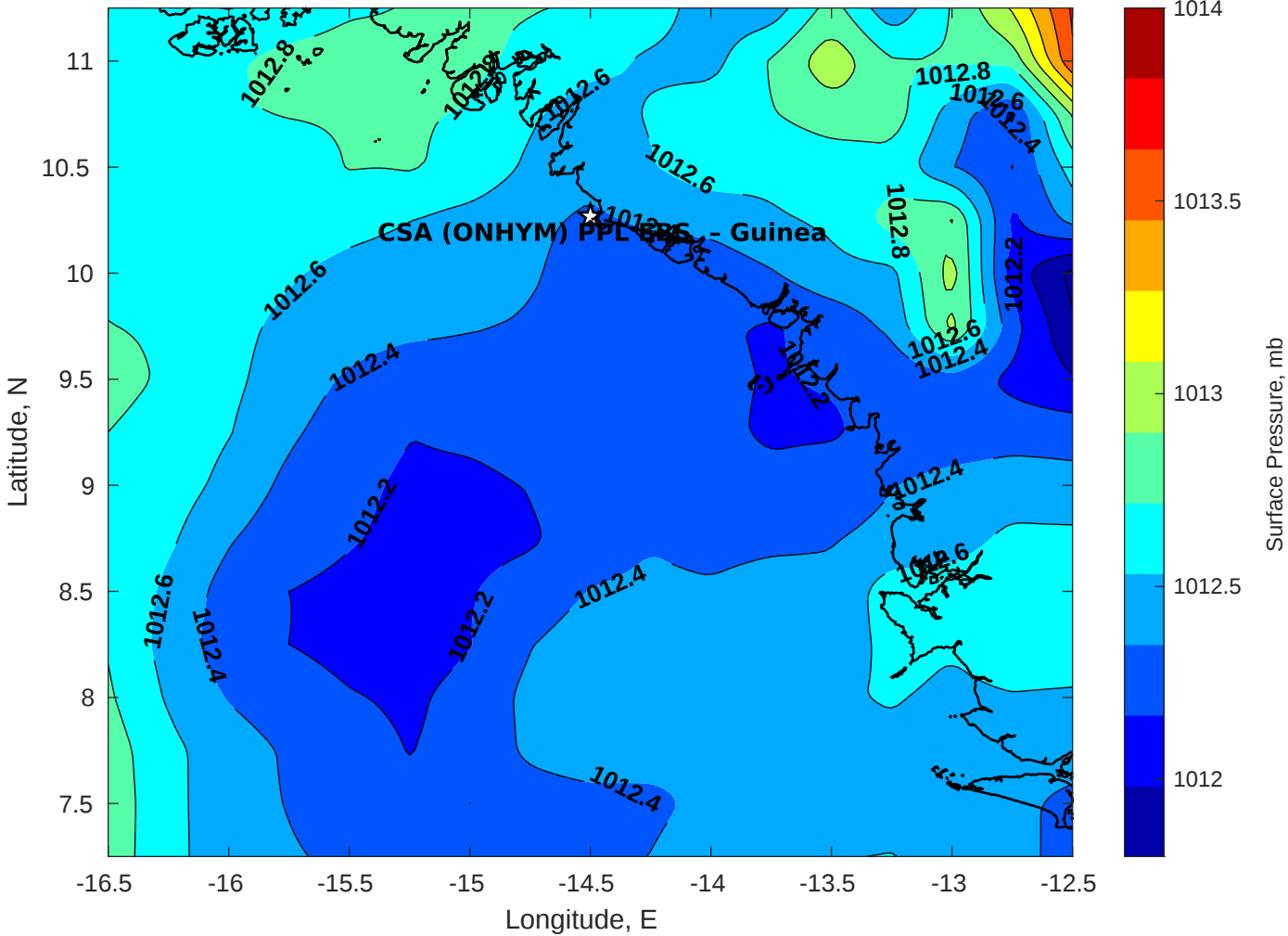
Surface Pressure (mb) for CSA (ONHYM) PPL EBS - Guinea at 16-Apr-2025 00:00:00
