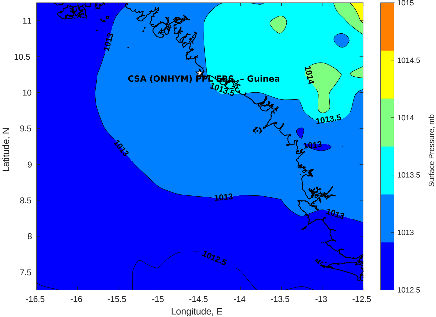
Surface Pressure (mb) for CSA (ONHYM) PPL EBS - Guinea at 18-Apr-2025 00:00:00
