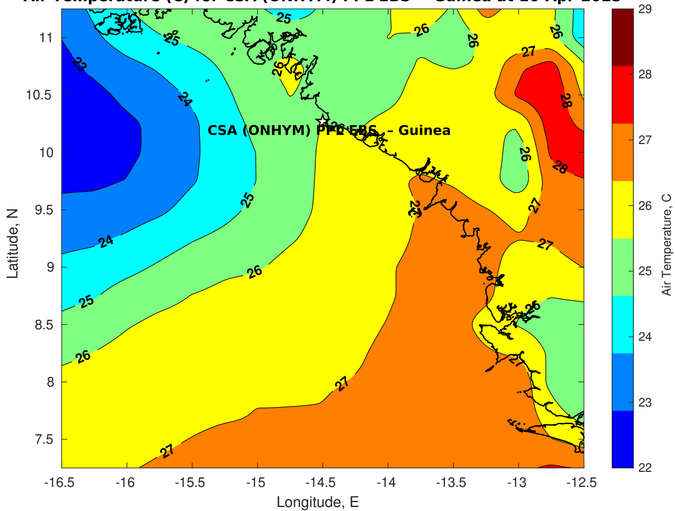
Air Temperature (C) for CSA (ONHYM) PPL EBS - Guinea at 16-Apr-2025
