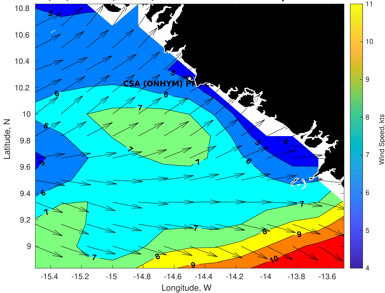
Winds (kts) for CSA (ONHYM) PPL EBS - Guinea at 16-Apr-2025 09:00:00
