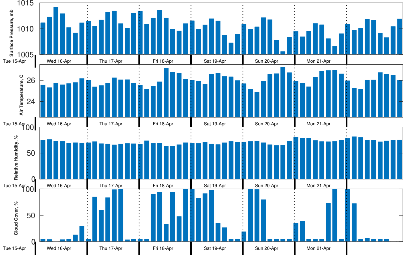
Met Forecast for CSA (ONHYM) PPL EBS - Guinea from 16-Apr-2025 00:00:00 to 23-Apr-2025 00:00:00
