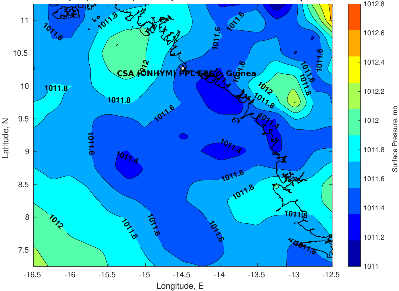
Surface Pressure (mb) for CSA (ONHYM) PPL EBS - Guinea at 17-Apr-2025 00:00:00
