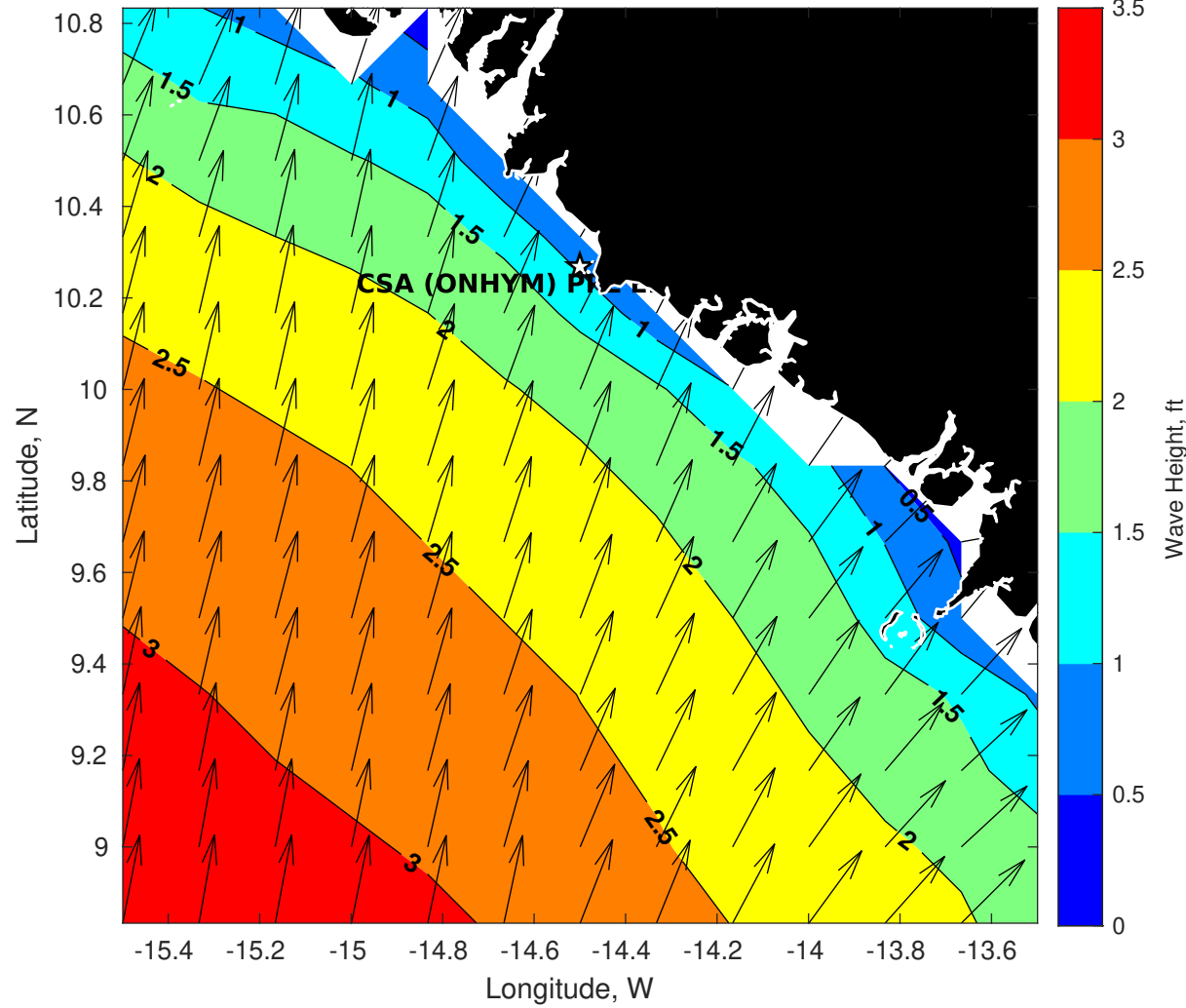
Wave Height (ft) for CSA (ONHYM) PPL EBS - Guinea at 16-Apr-2025 09:00:00
