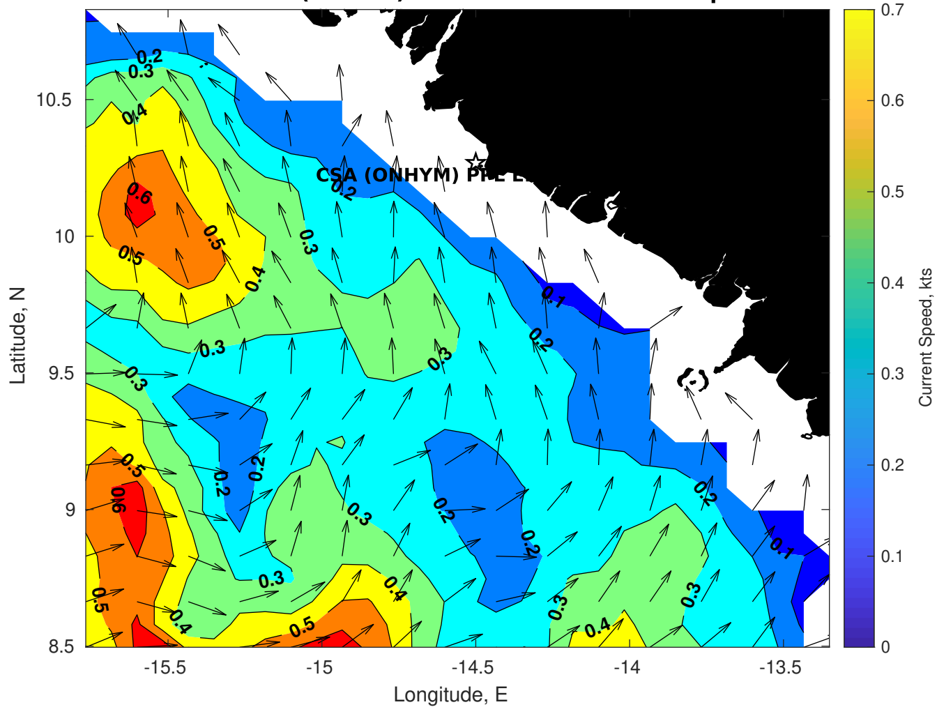
Surface Currents for CSA (ONHYM) PPL EBS - Guinea at 15-Apr-2025 00:00:00
