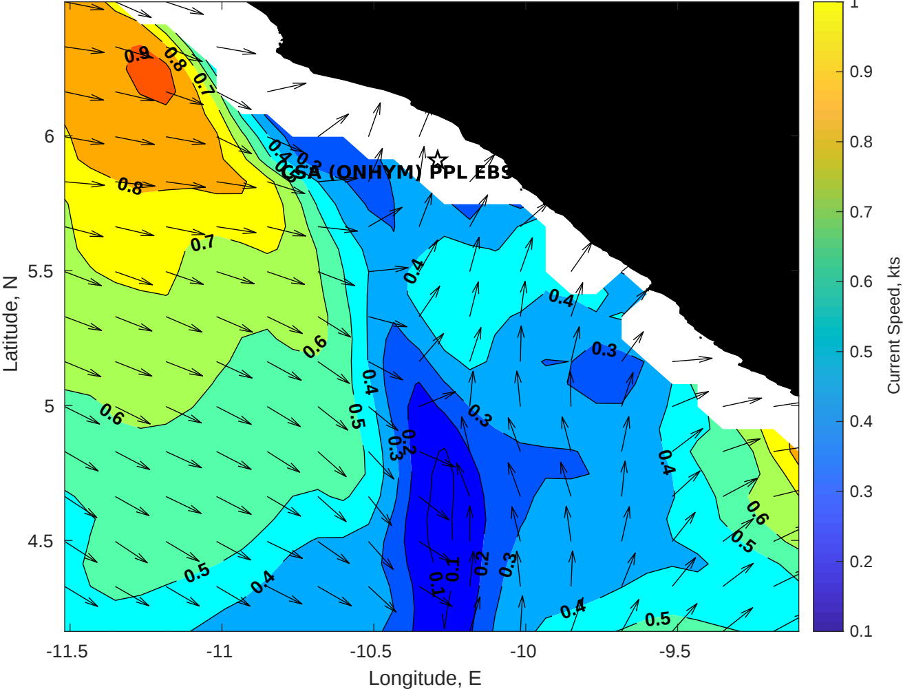
Surface Currents for CSA (ONHYM) PPL EBS - Liberia at 15-Apr-2025 00:00:00
