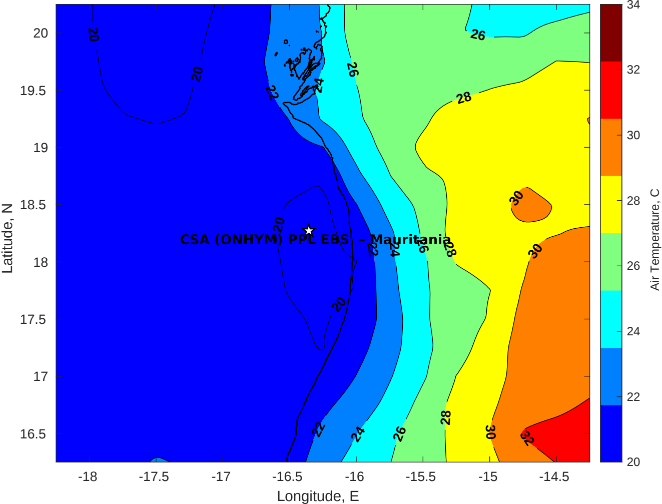
Air Temperature (C) for CSA (ONHYM) PPL EBS - Mauritania at 16-Apr-2025
