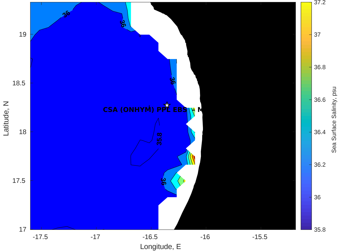
Surface Salinity for CSA (ONHYM) PPL EBS - Mauritania at 15-Apr-2025 00:00:00
