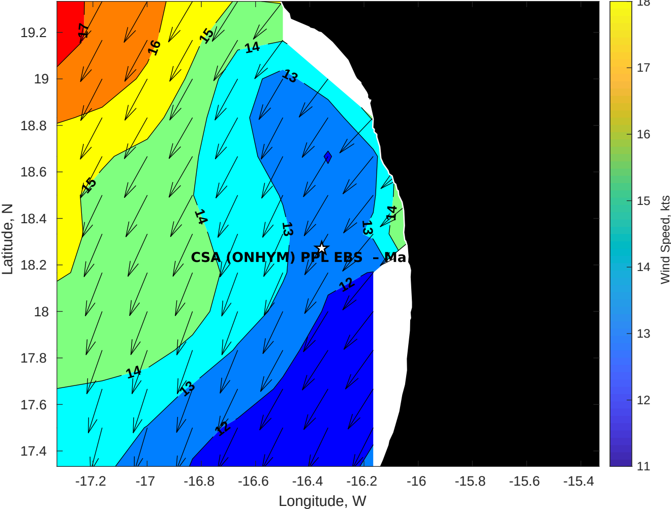
Winds (kts) for CSA (ONHYM) PPL EBS - Mauritania at 16-Apr-2025 09:00:00
