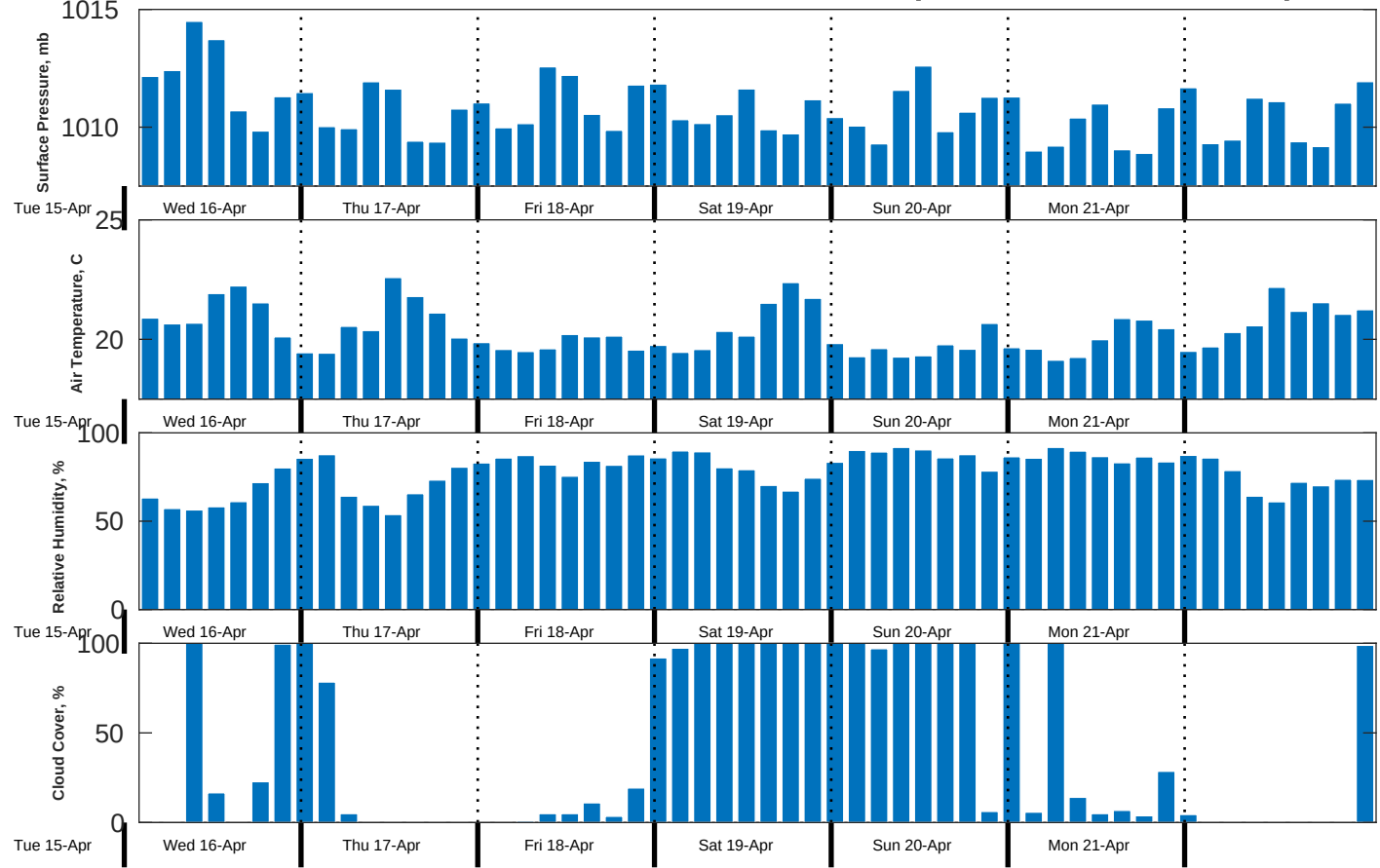
Met Forecast for CSA (ONHYM) PPL EBS - Mauritania from 16-Apr-2025 00:00:00 to 23-Apr-2025 00:00:00
