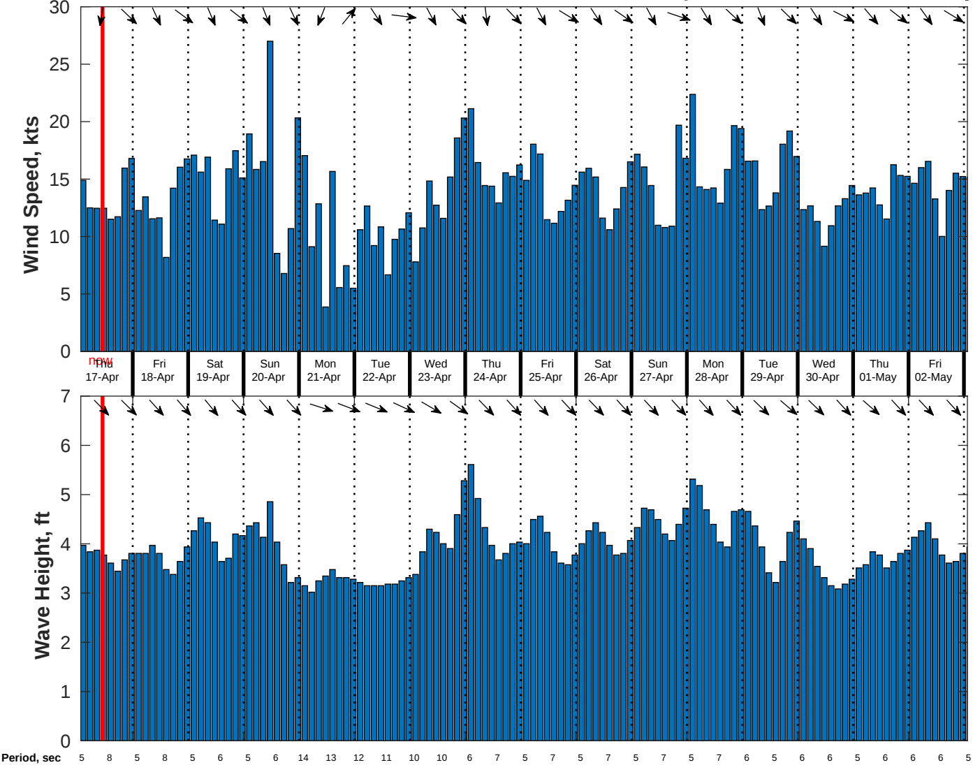
Wind & Wave Forecast for CSA (ONHYM) PPL EBS - Mauritania from 16-Apr-2025 01:00:00 to 02-May-2025 01:00:00
