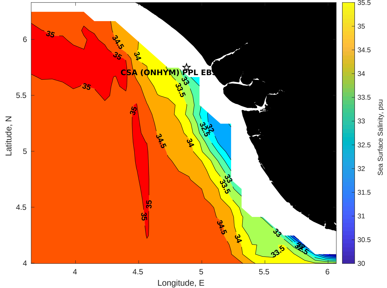
Surface Salinity for CSA (ONHYM) PPL EBS - Nigeria at 15-Apr-2025 00:00:00
