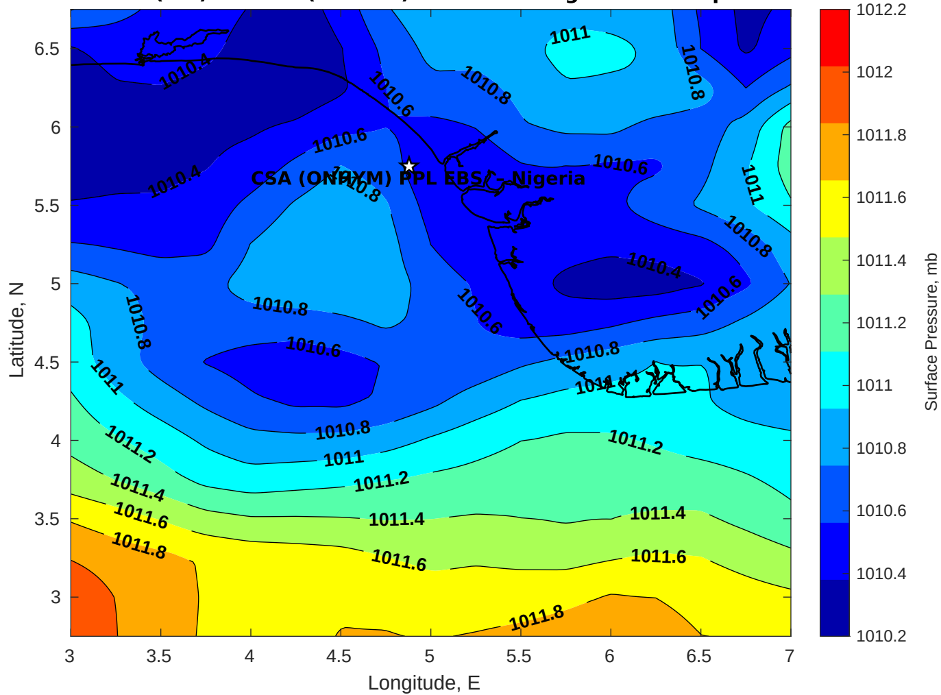
Surface Pressure (mb) for CSA (ONHYM) PPL EBS - Nigeria at 17-Apr-2025 00:00:00
