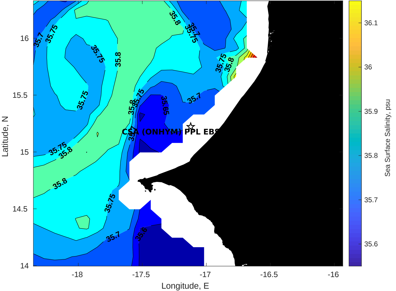
Surface Salinity for CSA (ONHYM) PPL EBS - Senegal at 15-Apr-2025 00:00:00
