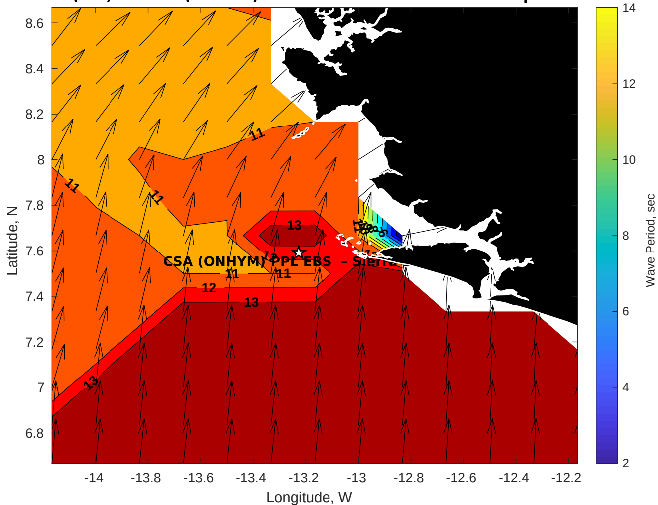
Wave Period (sec) for CSA (ONHYM) PPL EBS - Sierra Leone at 16-Apr-2025 09:00:00
