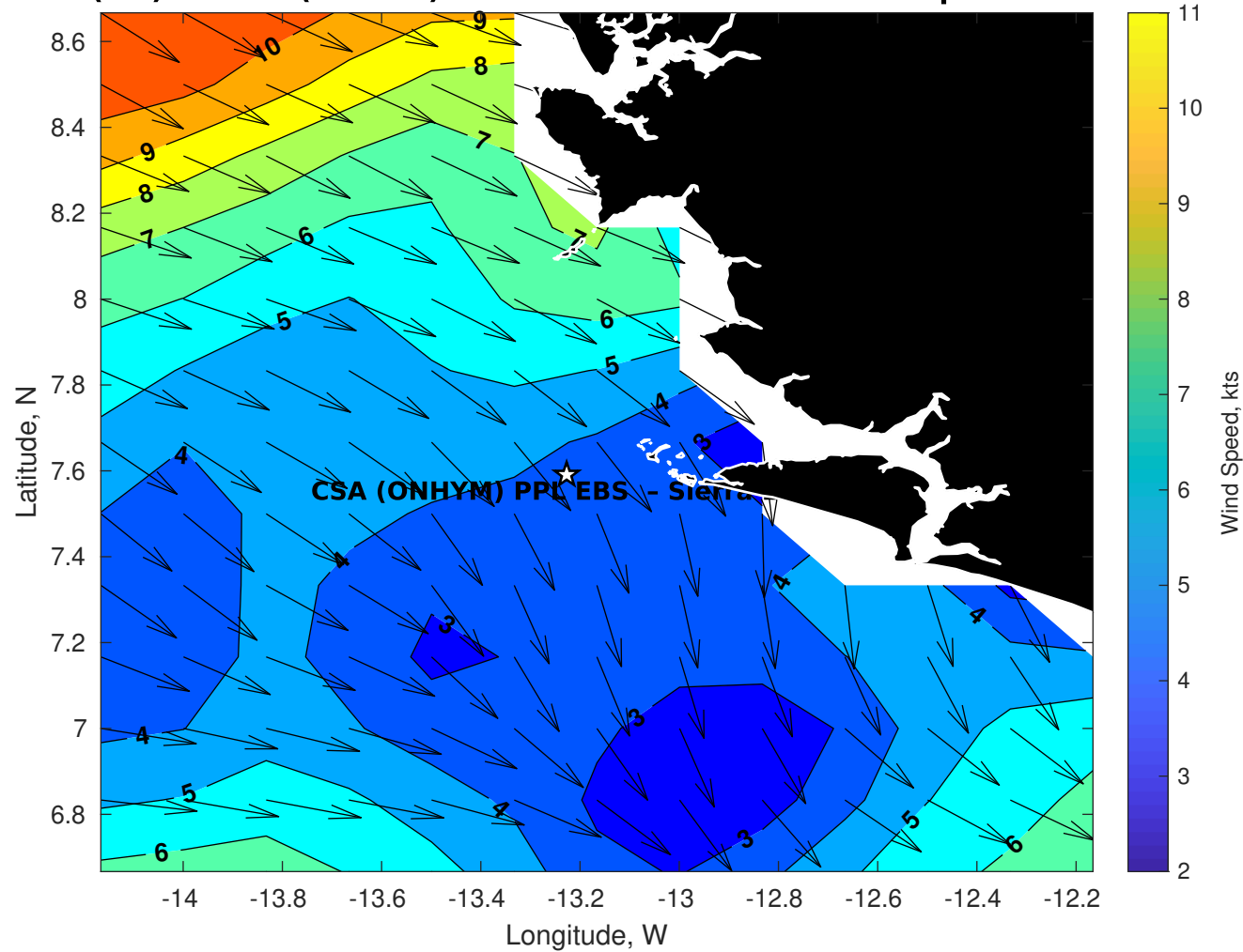
Winds (kts) for CSA (ONHYM) PPL EBS - Sierra Leone at 16-Apr-2025 09:00:00
