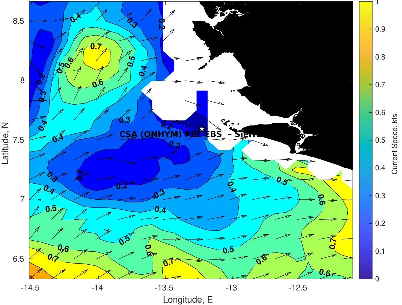
Surface Currents for CSA (ONHYM) PPL EBS - Sierra Leone at 15-Apr-2025 00:00:00
