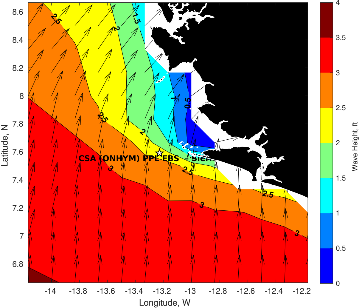
Wave Height (ft) for CSA (ONHYM) PPL EBS - Sierra Leone at 16-Apr-2025 09:00:00
