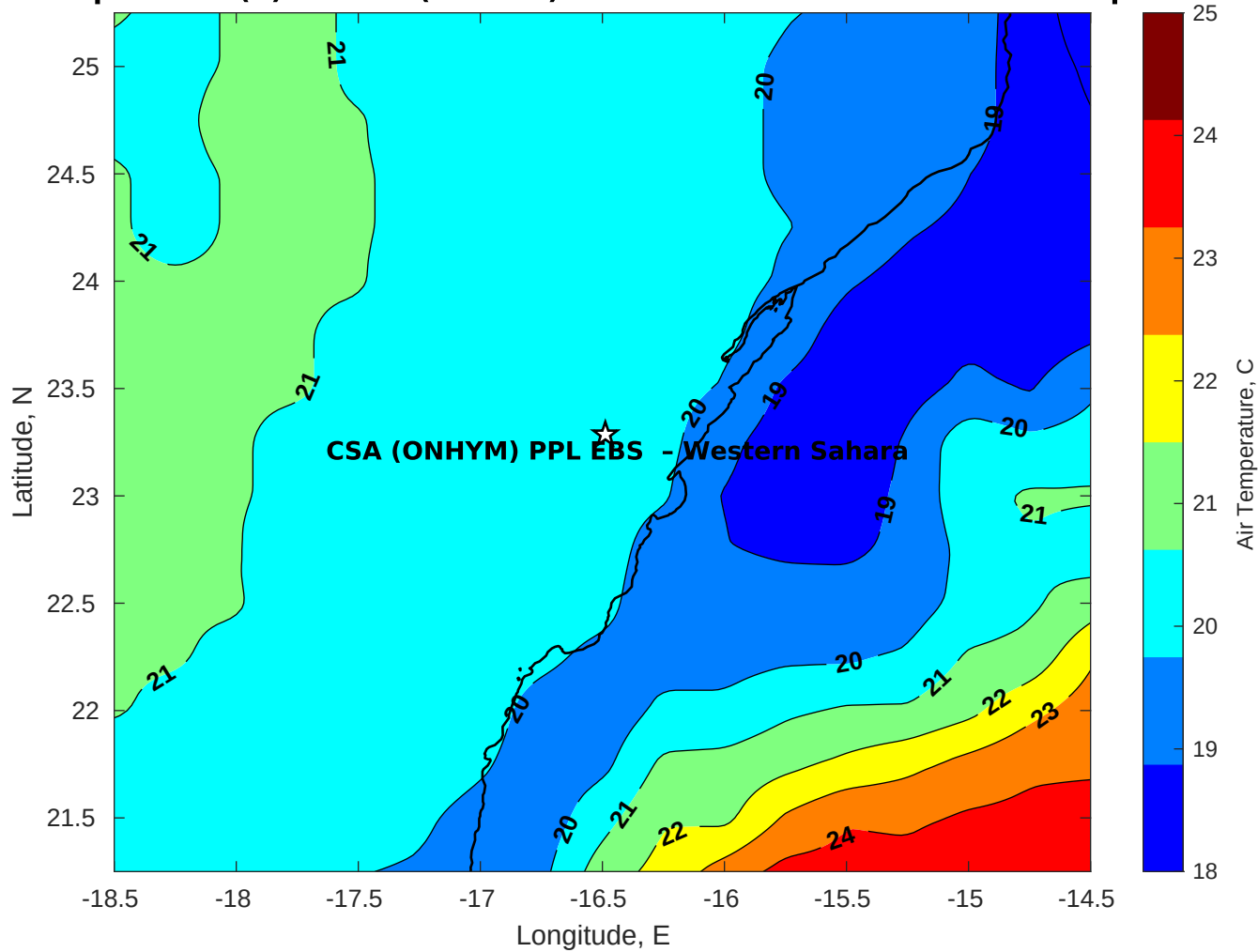
Air Temperature (C) for CSA (ONHYM) PPL EBS - Western Sahara at 16-Apr-2025
