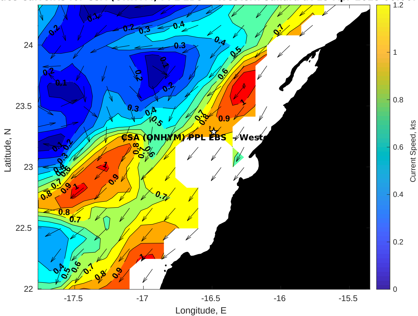
Surface Currents for CSA (ONHYM) PPL EBS - Western Sahara at 15-Apr-2025 00:00:00
