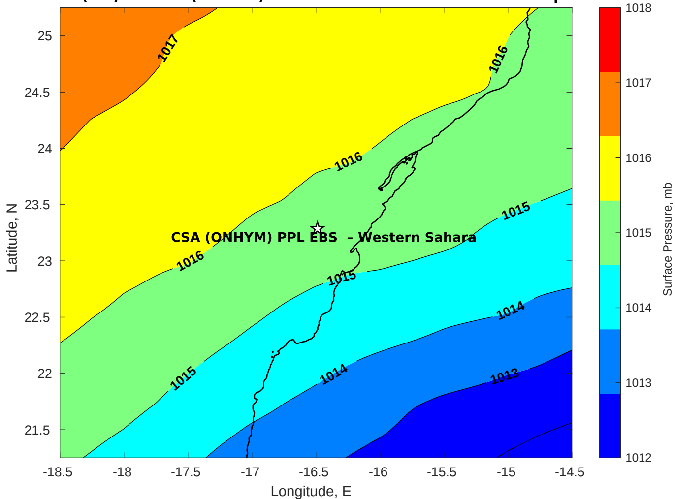
Surface Pressure (mb) for CSA (ONHYM) PPL EBS - Western Sahara at 18-Apr-2025 00:00:00
