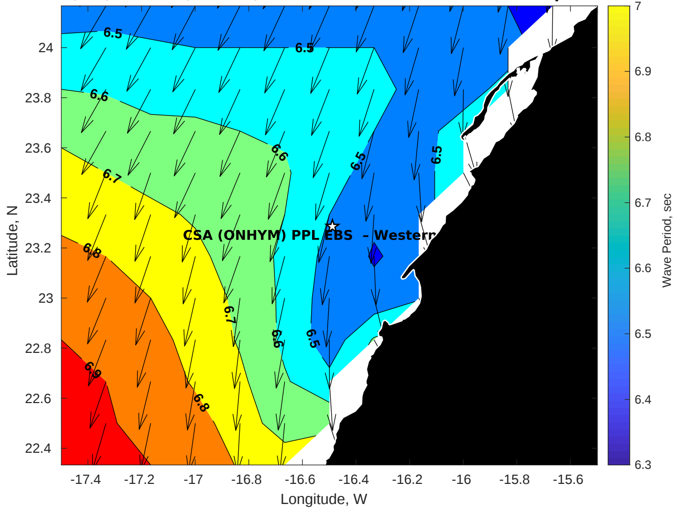
Wave Period (sec) for CSA (ONHYM) PPL EBS - Western Sahara at 16-Apr-2025 09:00:00
