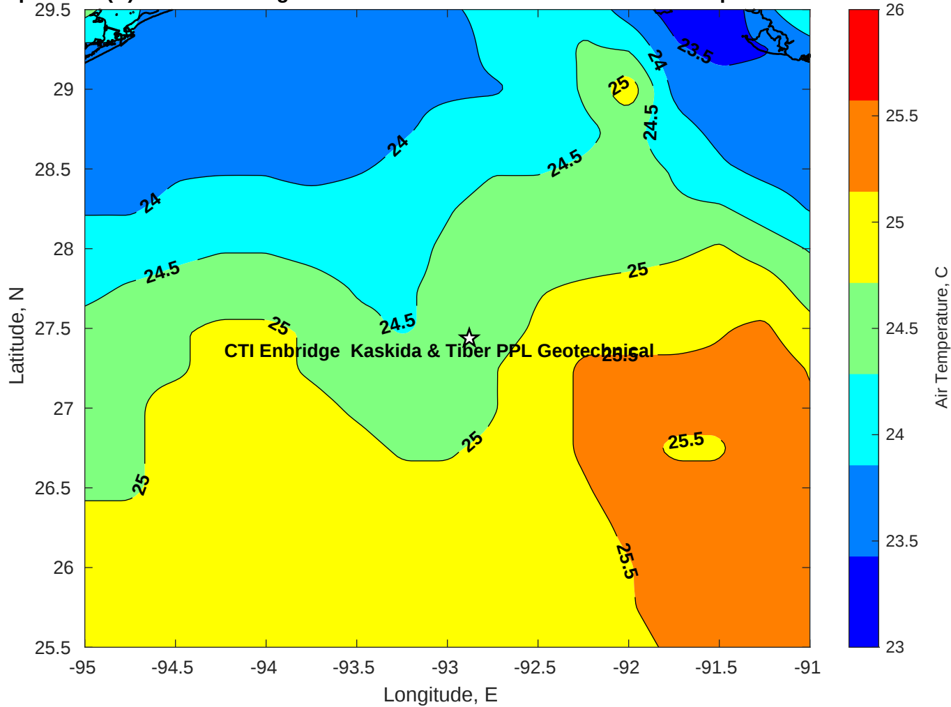
Air Temperature (C) for CTI Enbridge Kaskida & Tiber PPL Geotechnical at 16-Apr-2025
