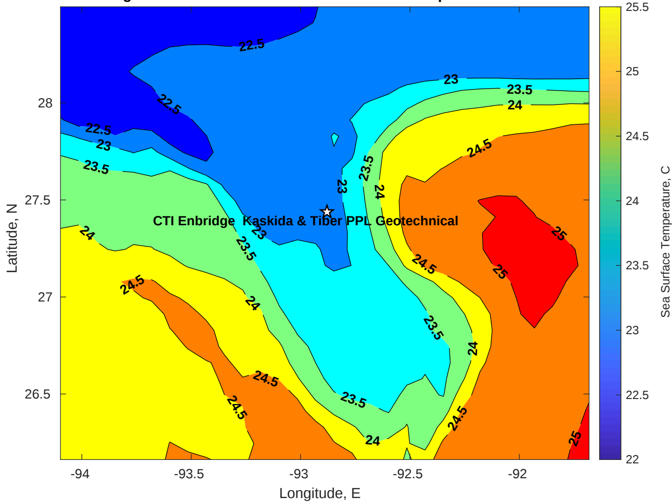
SST for CTI Enbridge Kaskida & Tiber PPL Geotechnical at 15-Apr-2025 00:00:00
