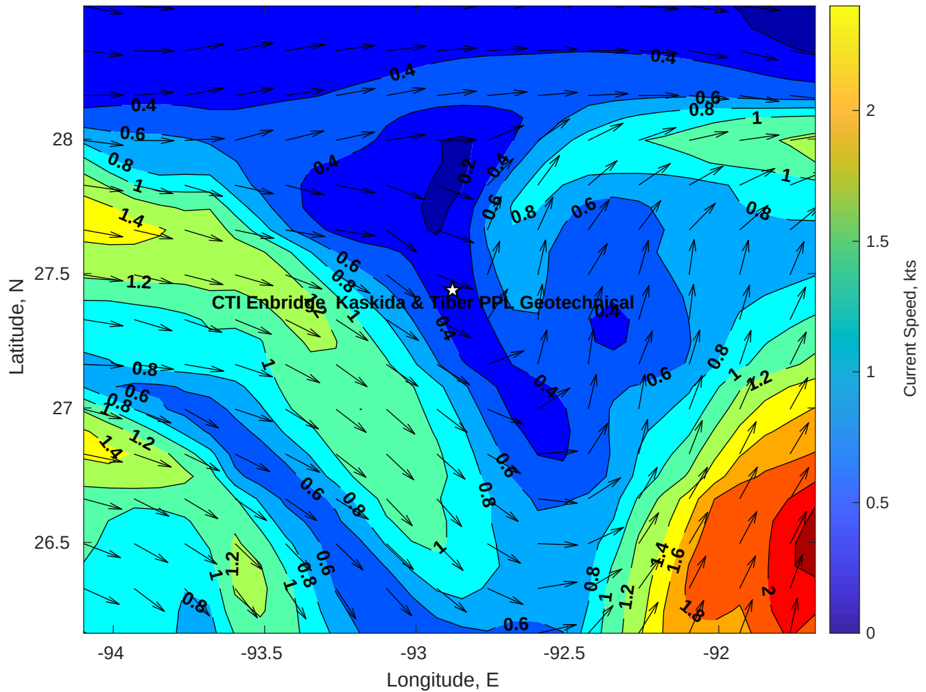
Surface Currents for CTI Enbridge Kaskida & Tiber PPL Geotechnical at 15-Apr-2025 00:00:00
