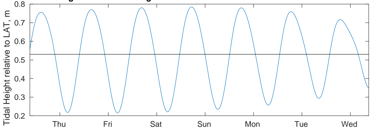
Tidal Currents and Heights for CTI Enbridge Kaskida & Tiber PPL Geotechnical at 20250416
