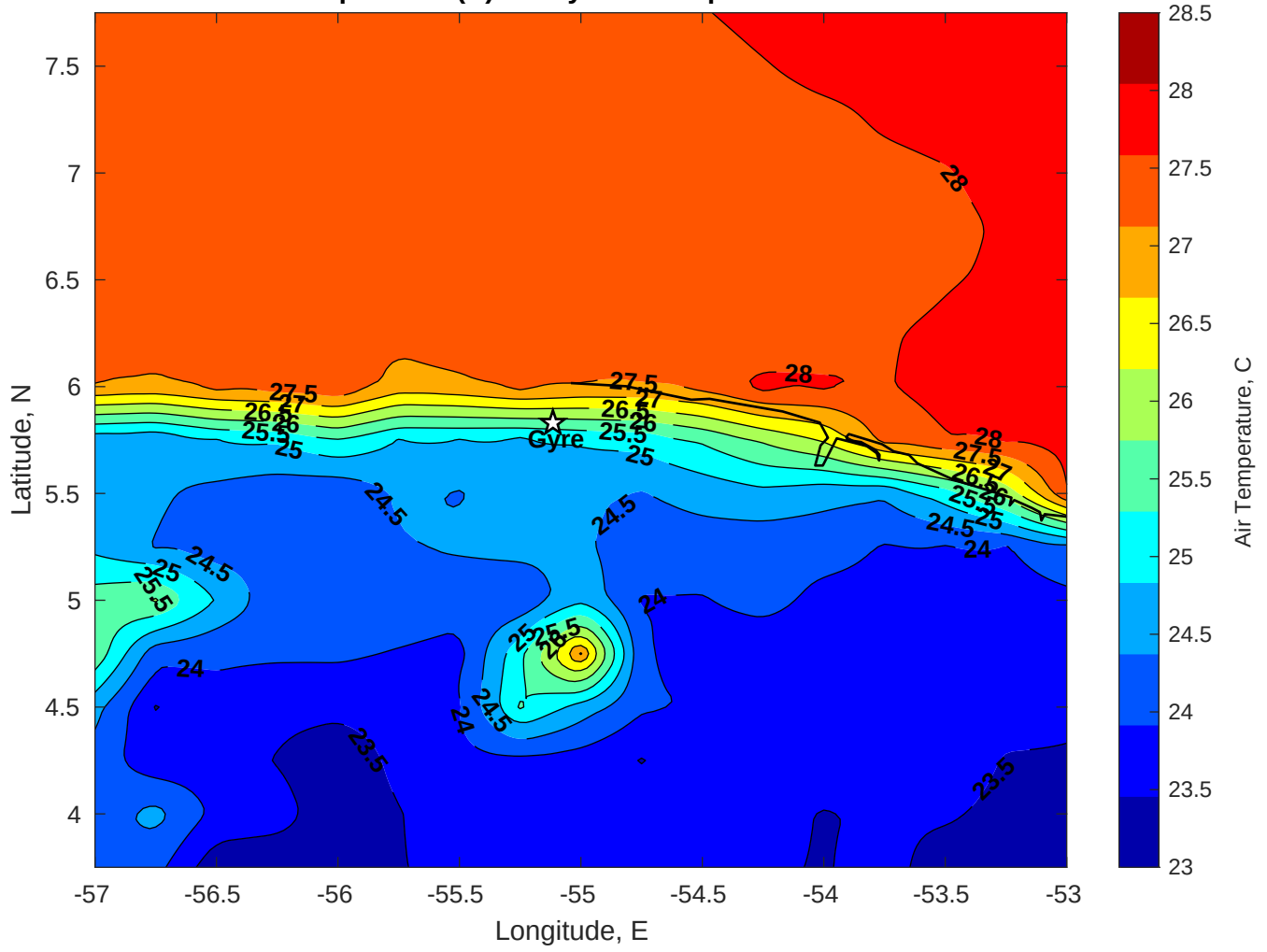
Air Temperature (C) for Gyre at 16-Apr-2025
