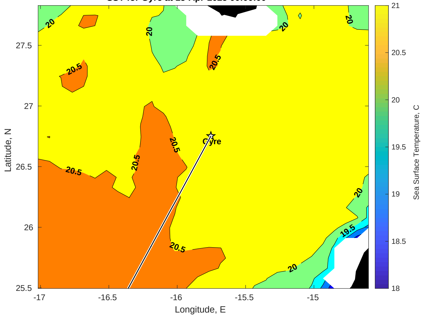
SST for Gyre at 15-Apr-2025 00:00:00
