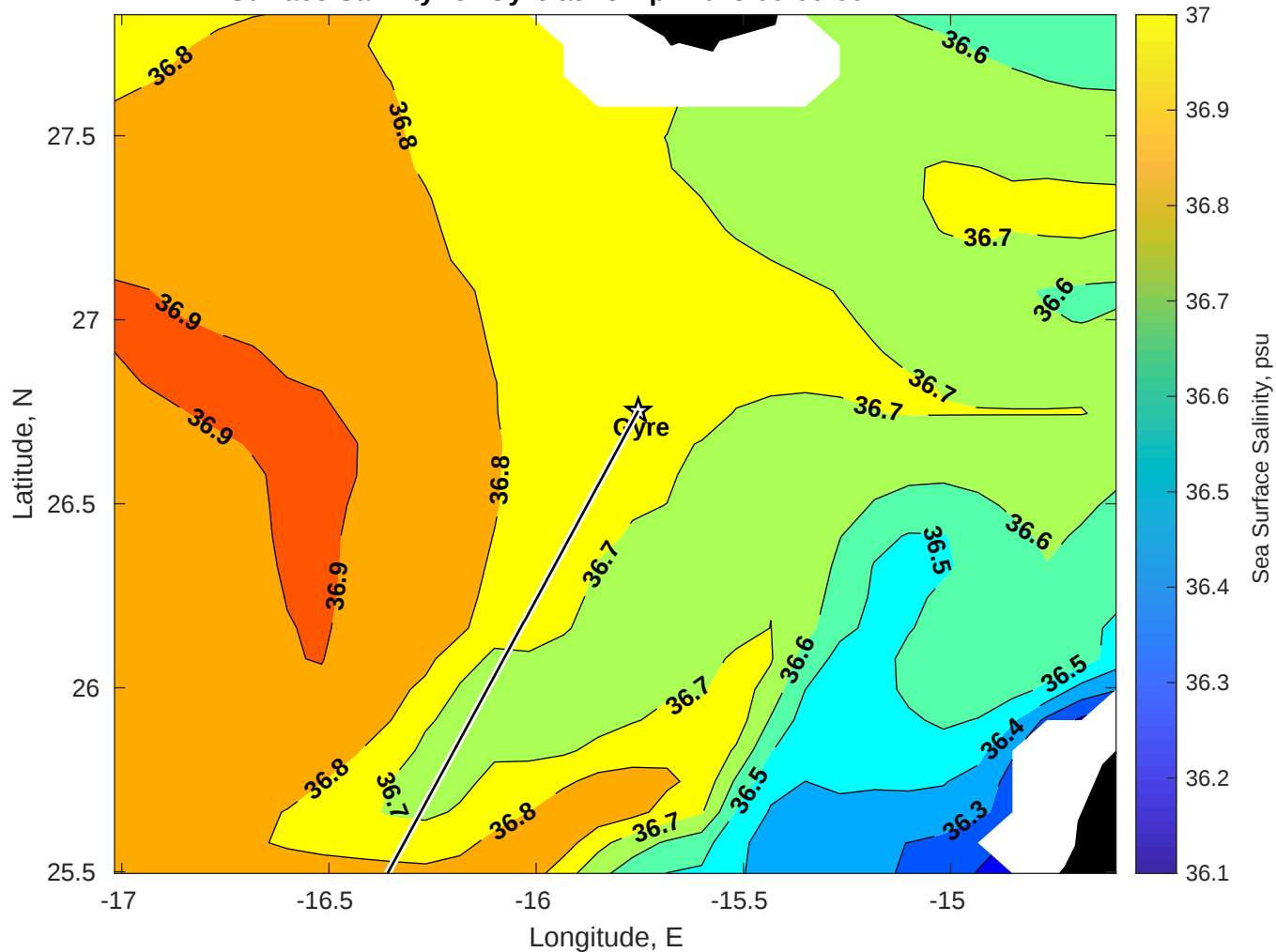
Surface Salinity for Gyre at 15-Apr-2025 00:00:00
