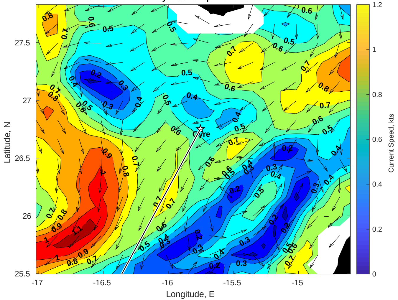
Surface Currents for Gyre at 15-Apr-2025 00:00:00
