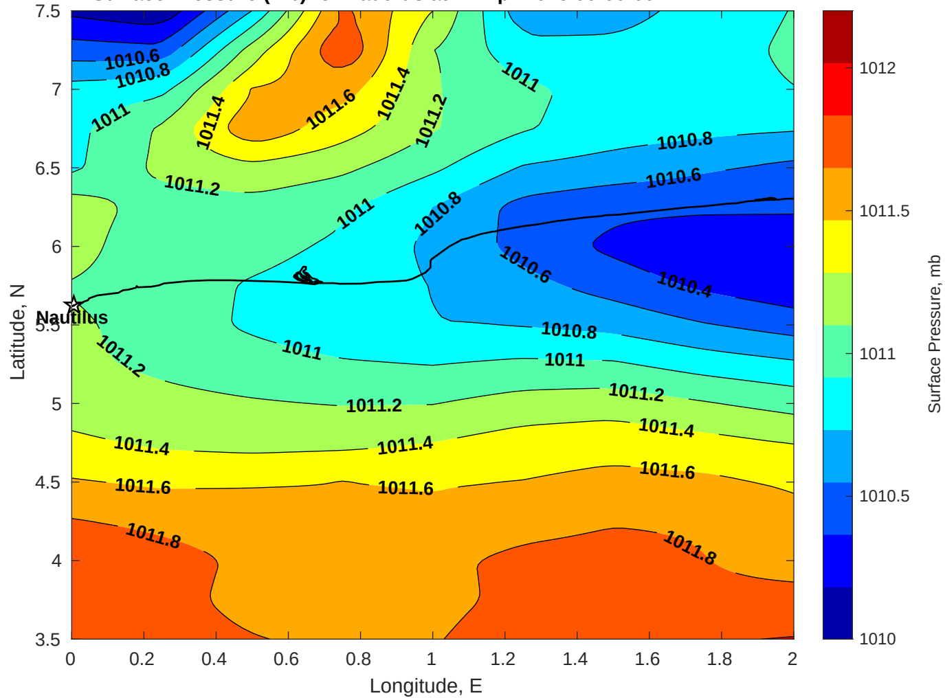
Surface Pressure (mb) for Nautilus at 17-Apr-2025 00:00:00
