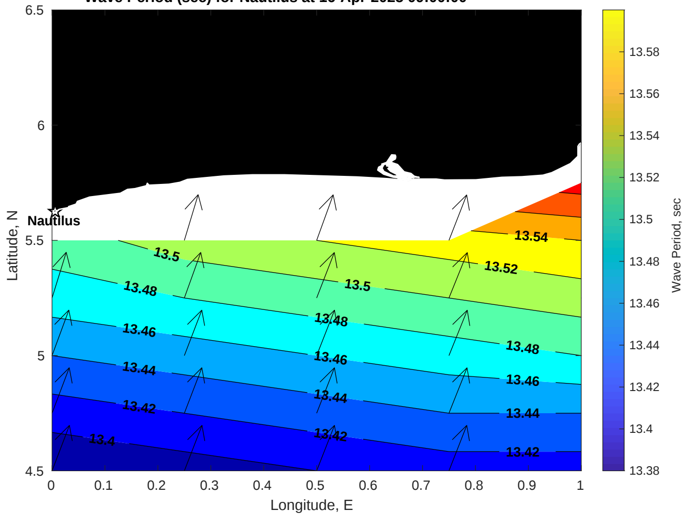
Wave Period (sec) for Nautilus at 16-Apr-2025 09:00:00
