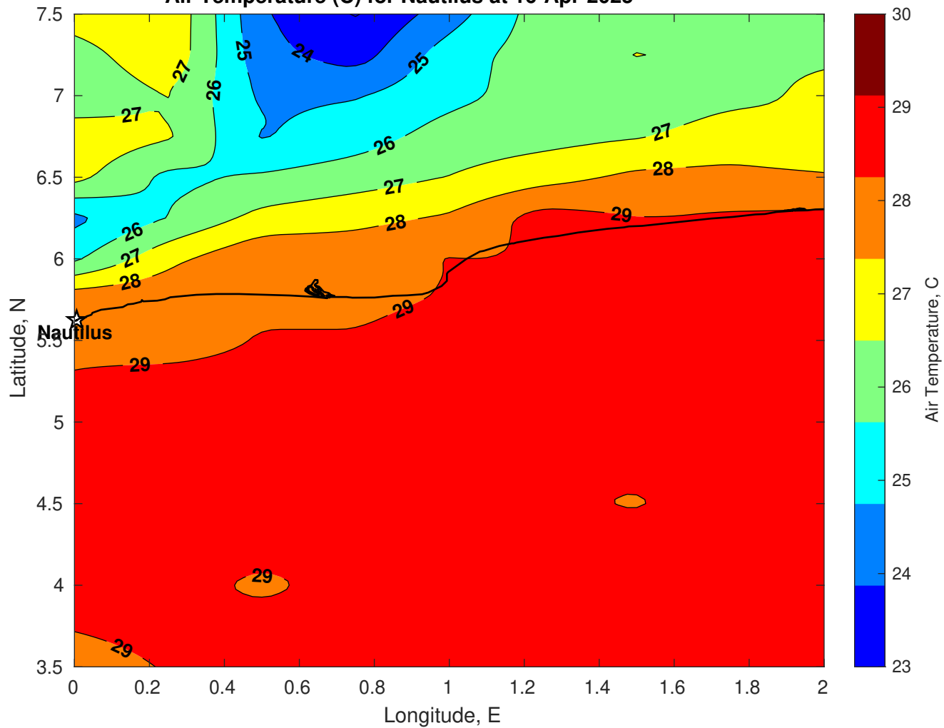
Air Temperature (C) for Nautilus at 16-Apr-2025
