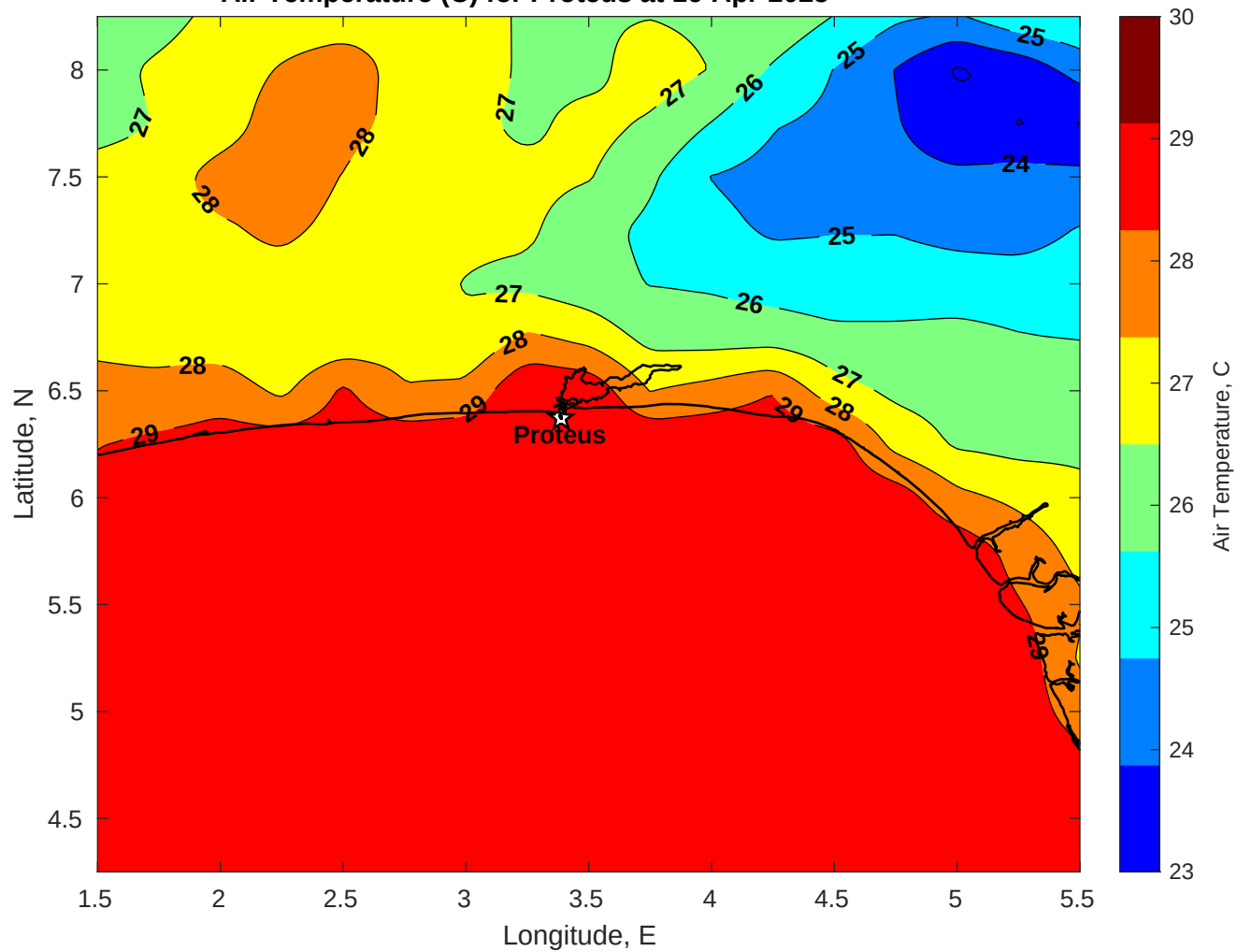
Air Temperature (C) for Proteus at 16-Apr-2025
