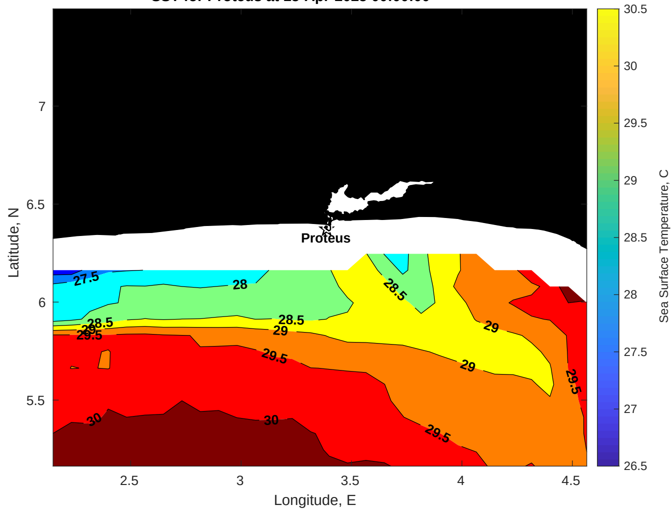
SST for Proteus at 15-Apr-2025 00:00:00
