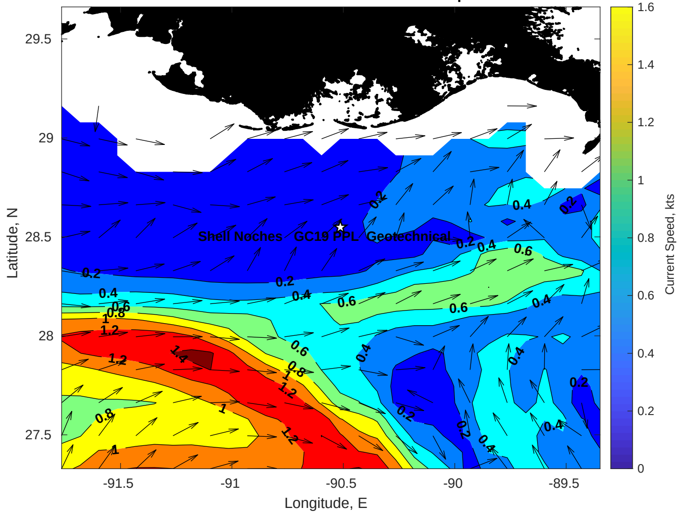
Surface Currents for Shell Noches GC19 PPL Geotechnical at 15-Apr-2025 00:00:00
