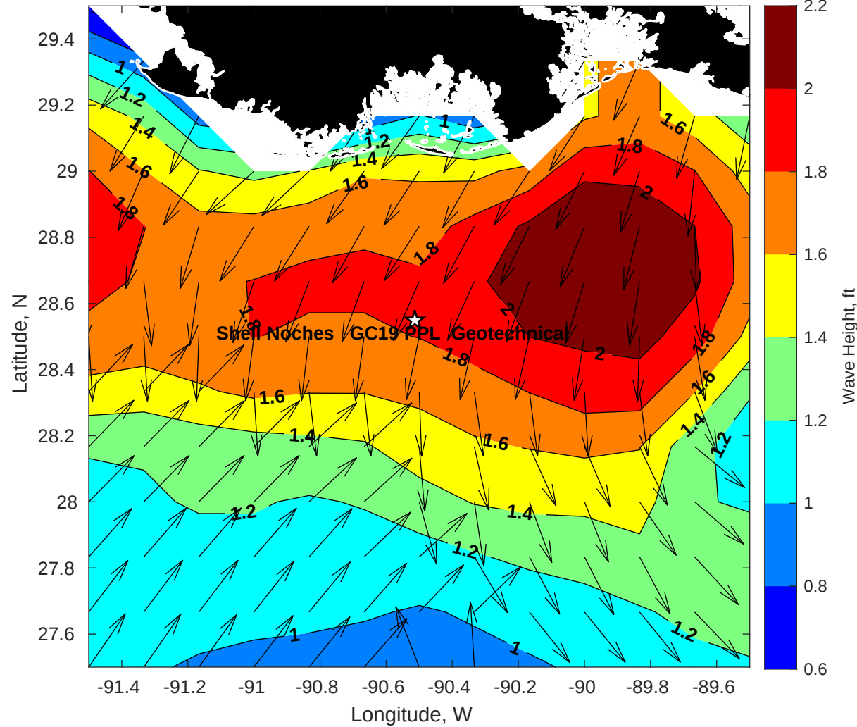
Wave Height (ft) for Shell Noches GC19 PPL Geotechnical at 16-Apr-2025 09:00:00
