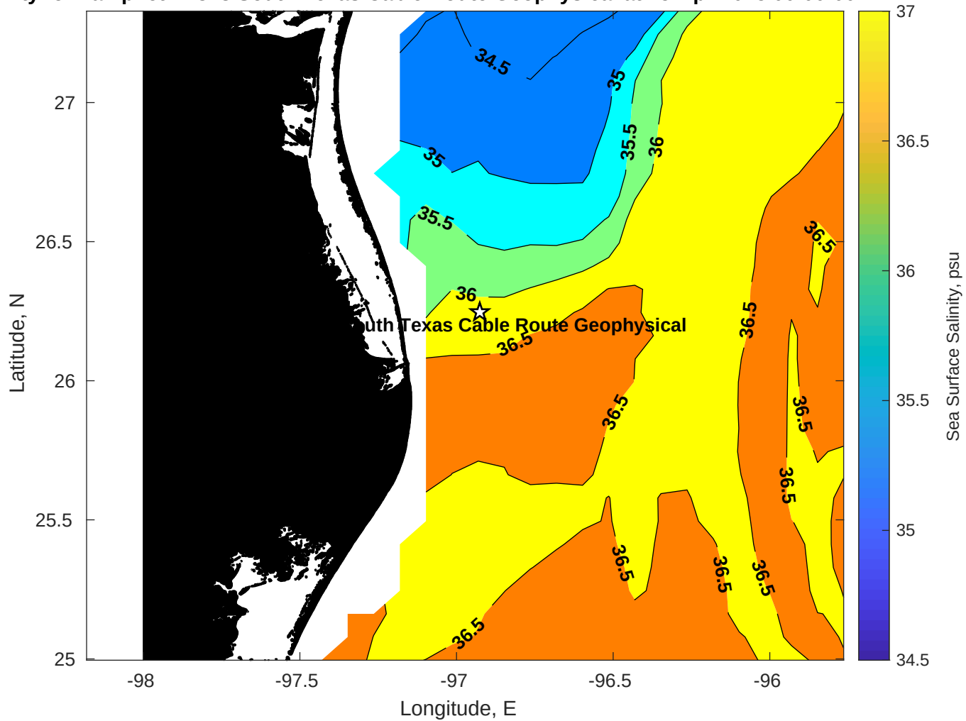
Surface Salinity for Tampnet P2378 South Texas Cable Route Geophysical at 15-Apr-2025 00:00:00
