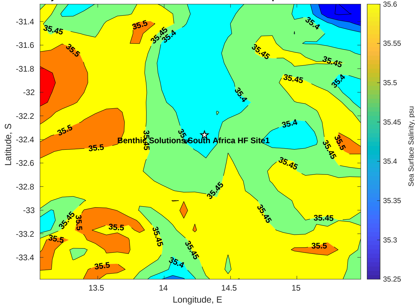
Surface Salinity for Benthic Solutions South Africa HF Site1 at 16-Apr-2025 00:00:00
