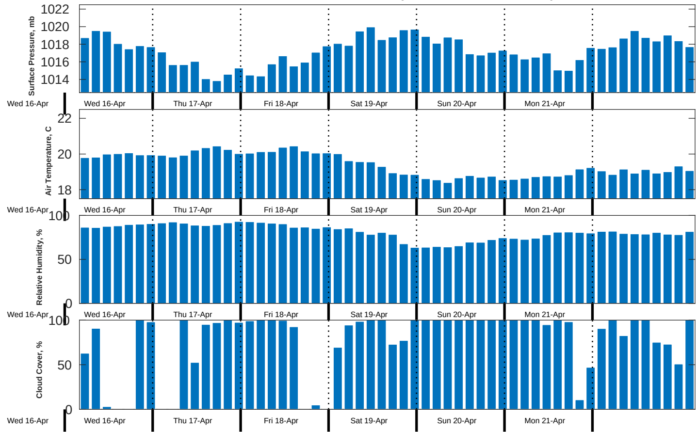
Met Forecast for Benthic Solutions South Africa HF Site1 from 17-Apr-2025 00:00:00 to 24-Apr-2025 00:00:00
